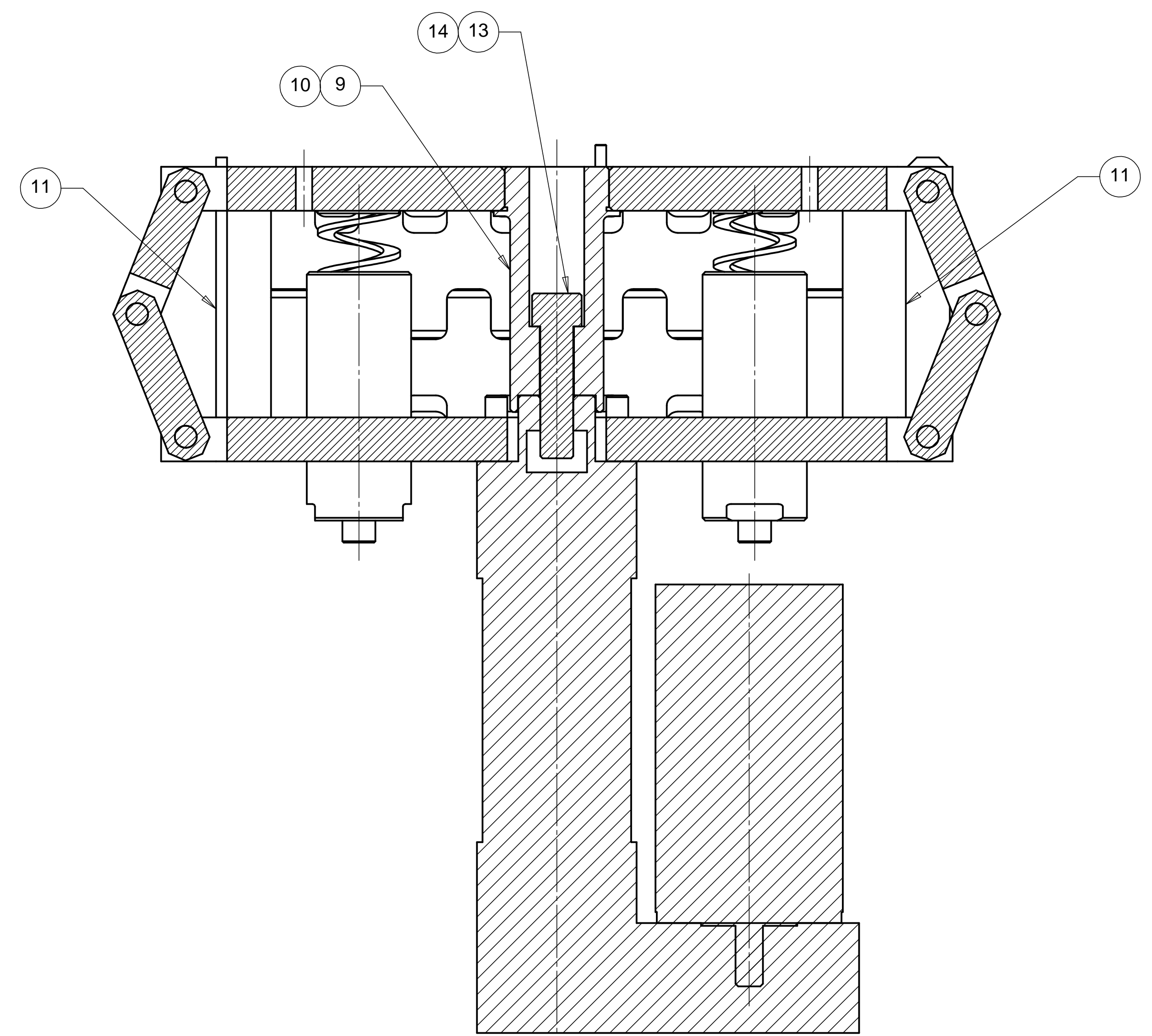
SECTION THRU DRIVE SHAFT
