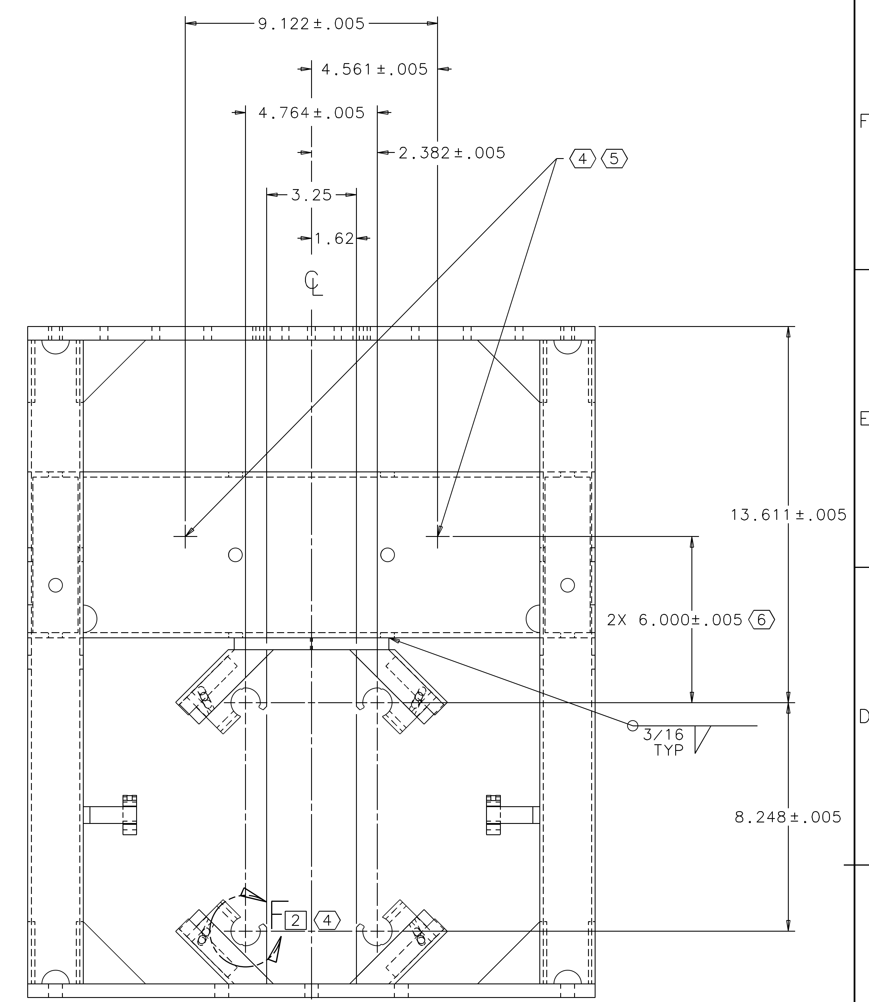
VIEW B-B 1
