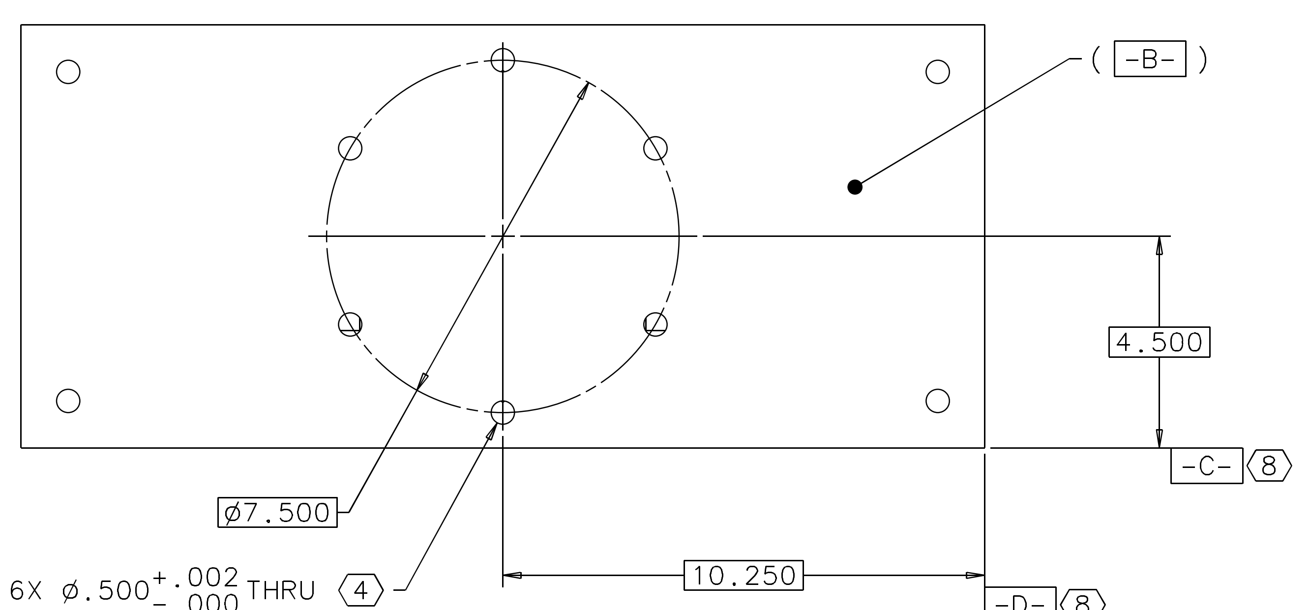
VIEW C-C 1
