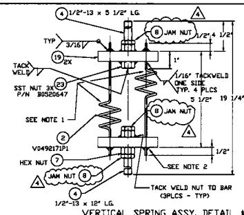
VERTICAL SPRING ASSY. DETAIL #1
