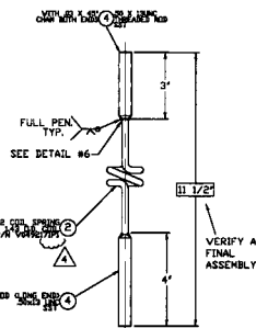
DETAIL #2 2 REQUIRED
