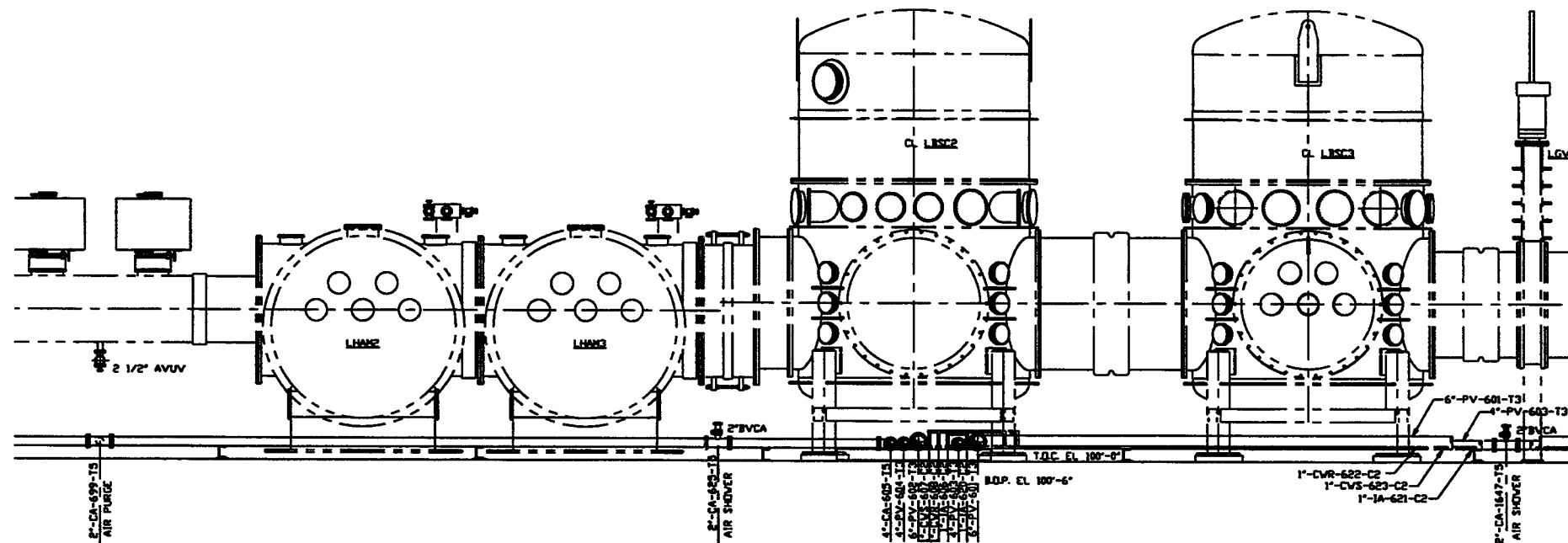
ELEVATION K V049-5-040, SHT.1
