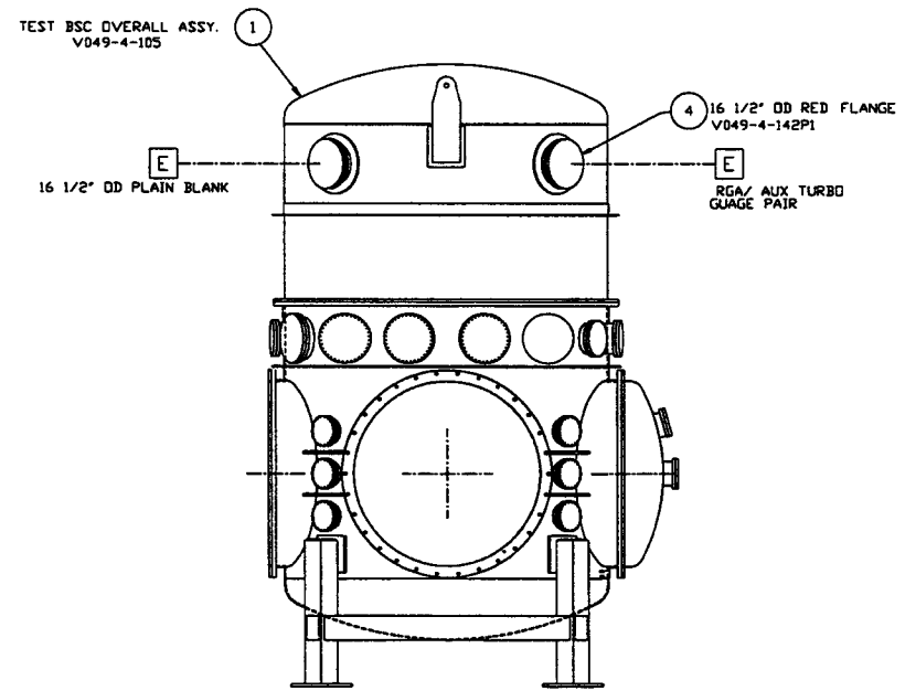
ELEVATION VIEW @ 180°
