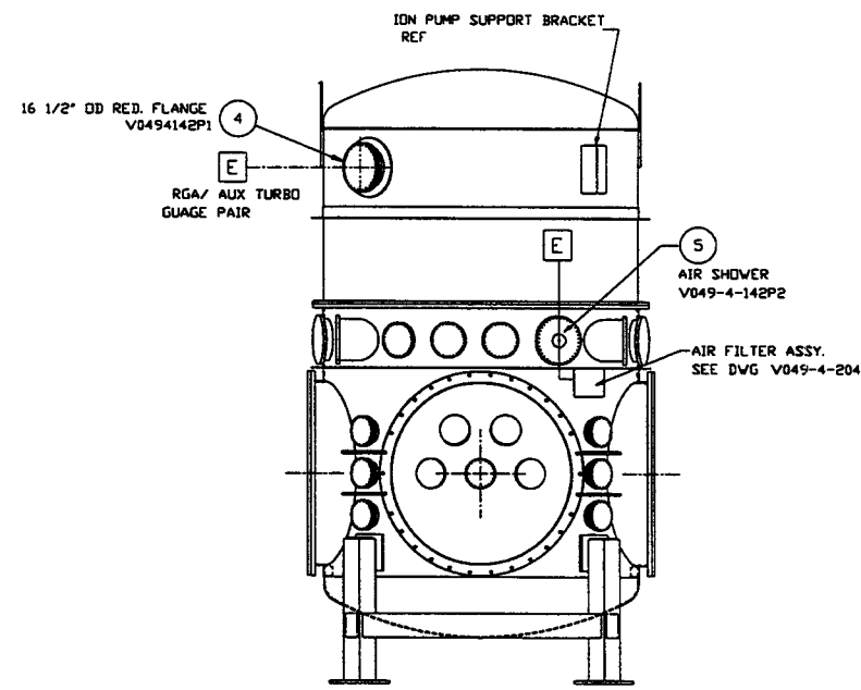
ELEVATION VIEW @ 90°
