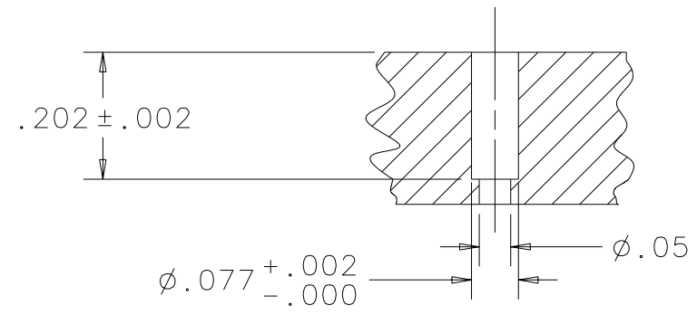
VIEW A SCALE 4/1 25X
