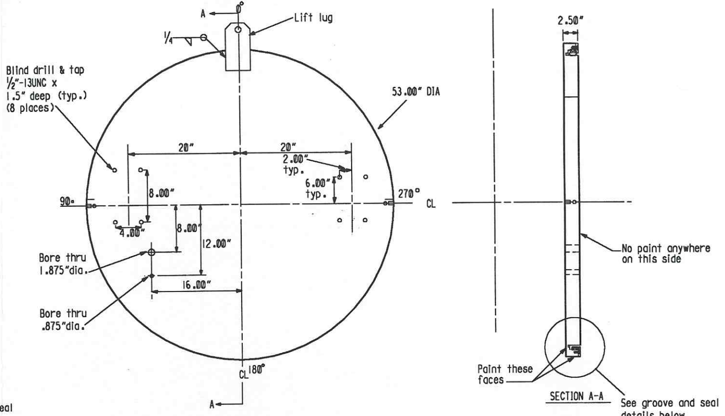
LEAK TEST HEAD (BLIND END) (THREE HEADS REQ'D)
