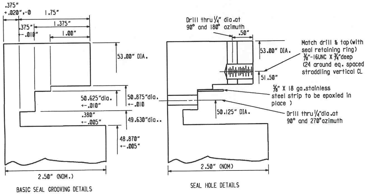
GROOVE AND SEAL DETAILS
