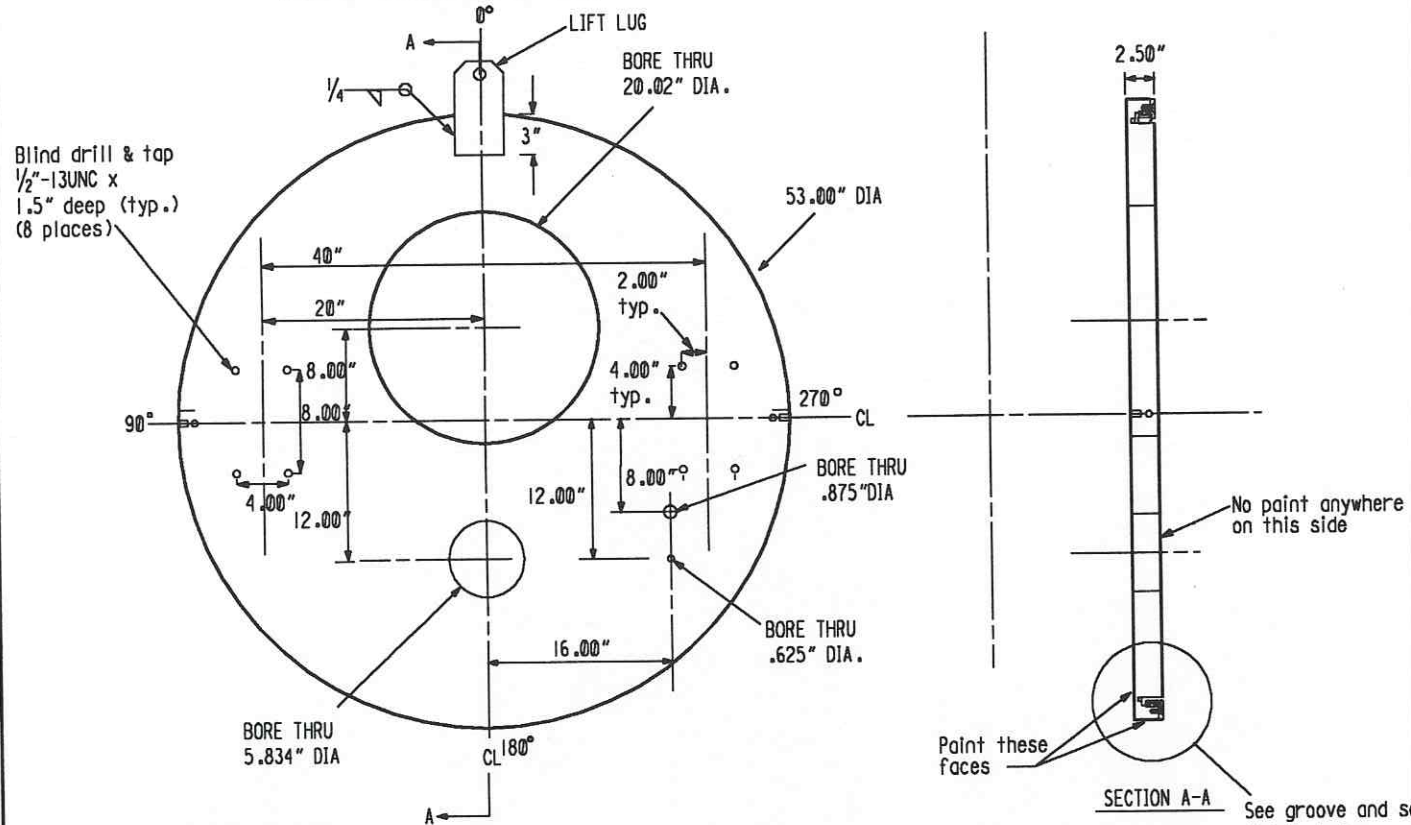
LEAK TEST HEAD (PUMP END) (THREE HEADS REQ'D)
