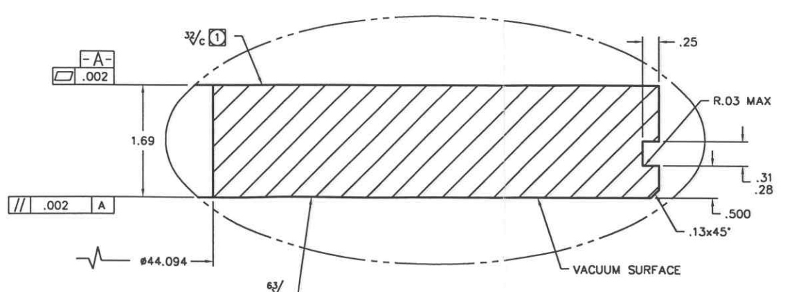
DETAIL #1 SCALE : NONE
