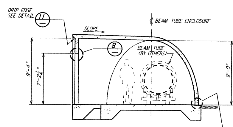
SECTION C \frac{3}{4}'' = 1'-0''
