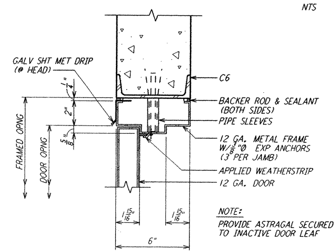
JAMB (HEAD SIM) DETAIL 9 3'' = 1'-0''
