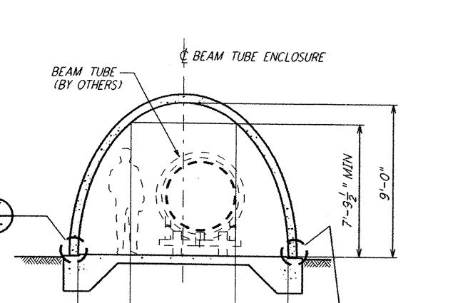
SECTION E \frac{3}{4}'' = 1'-0''
