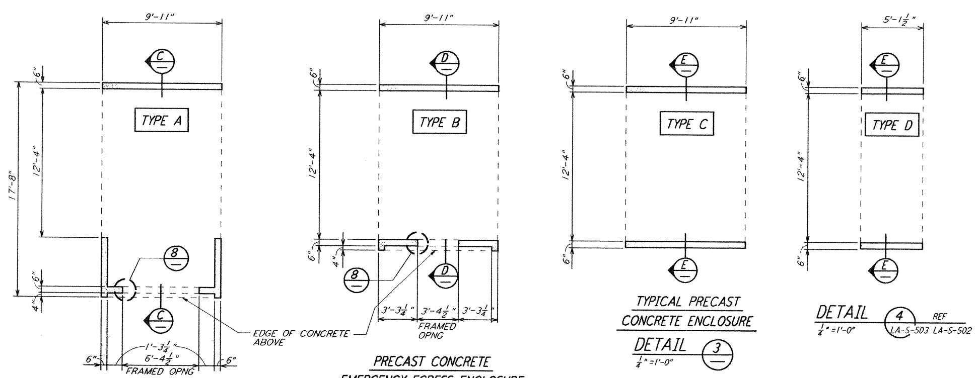
PRECAST CONCRETE SERVICE ENTRANCE ENCLOSURE DETAIL 1 \frac{3}{4}'' = 1'-0''
