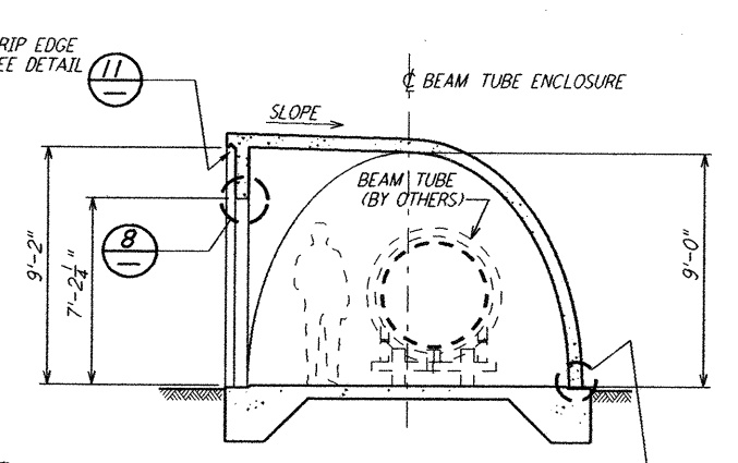
SECTION D \frac{3}{4}'' = 1'-0''
