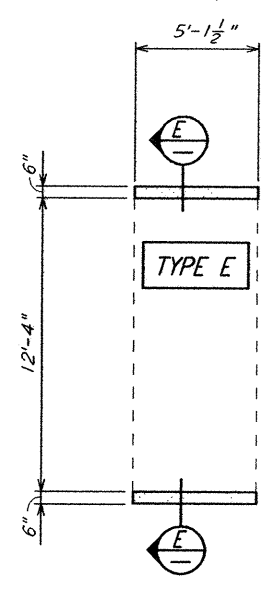
DETAIL 5 \frac{3}{4}'' = 1'-0'' REF LA-S-503 LA-S-502
