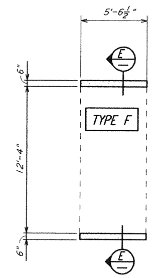
DETAIL 12 \frac{3}{4}'' = 1'-0'' REF LA-S-503 LA-S-502
