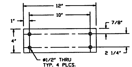
ITEM 2 MAT'L: 12" X 4" X 1/2" THK. SILICON PAD, 40 DUREMETER QTY: 2 REQ'D
