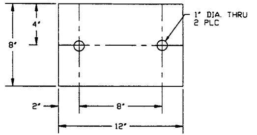
ITEM 1 MAT'L: 12" X 8" X 1" THK. A36 STL. PLATE QTY: 2 REQ'D
