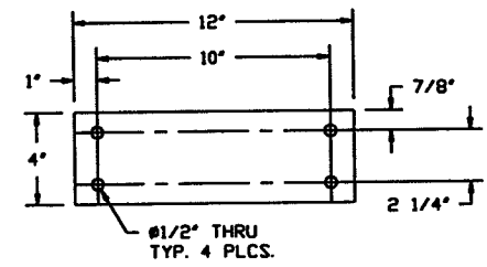
ITEM 2 MAT'L: 12" X 4" X 1/2" THK. SILICON PAD, 40 DUROMETER QTY: 2 REQ'D
