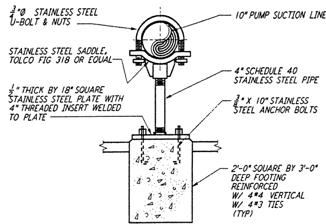
PIPE SUPPORT DETAIL 2 REF NTS (LA-P-411)
