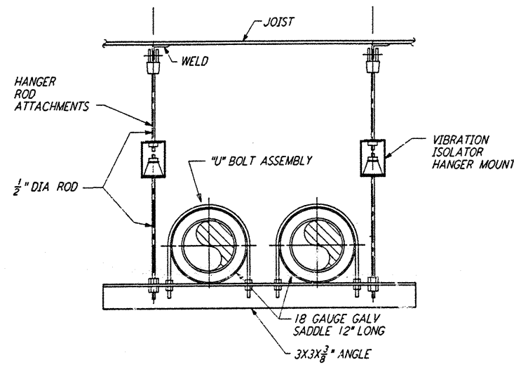
PIPE HANGER - TRAPEZE DETAIL 5 REF NTS (LA-P-411)
