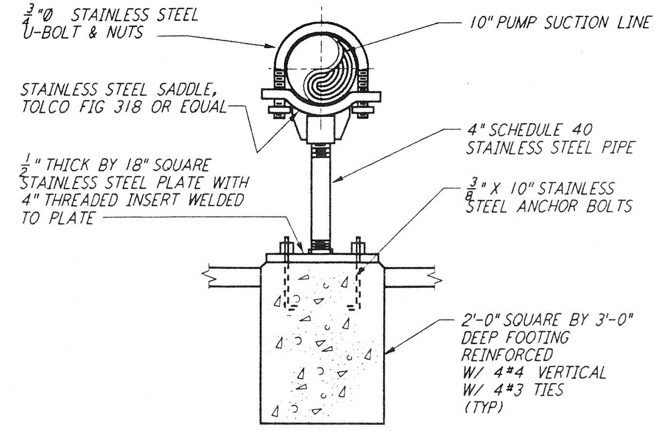
PIPE SUPPORT DETAIL (2) REF NTS LA-P-411
