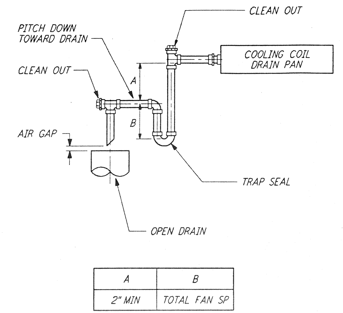
CONDENSATE DRAIN DETAIL (4) REF NTS LA-P-411
