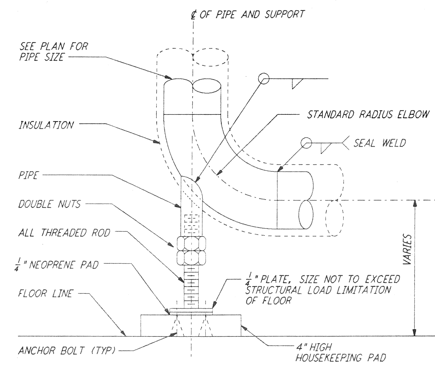
BASE ELBOW SUPPORT DETAIL (7) REF NTS LA-P-411
