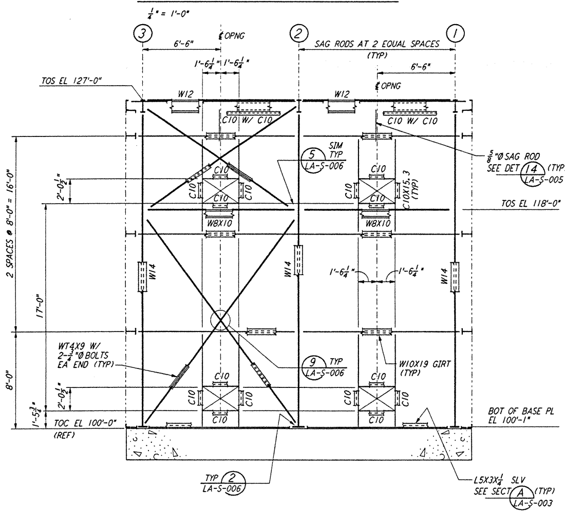
LOOKING SOUTH - FOR MID STATION "A" ON ARM 2 LOOKING EAST - FOR MID STATION "B" ON ARM 1 ELEVATION AT COLUMN LINE A \frac{1}{4}'' = 1'-0''
