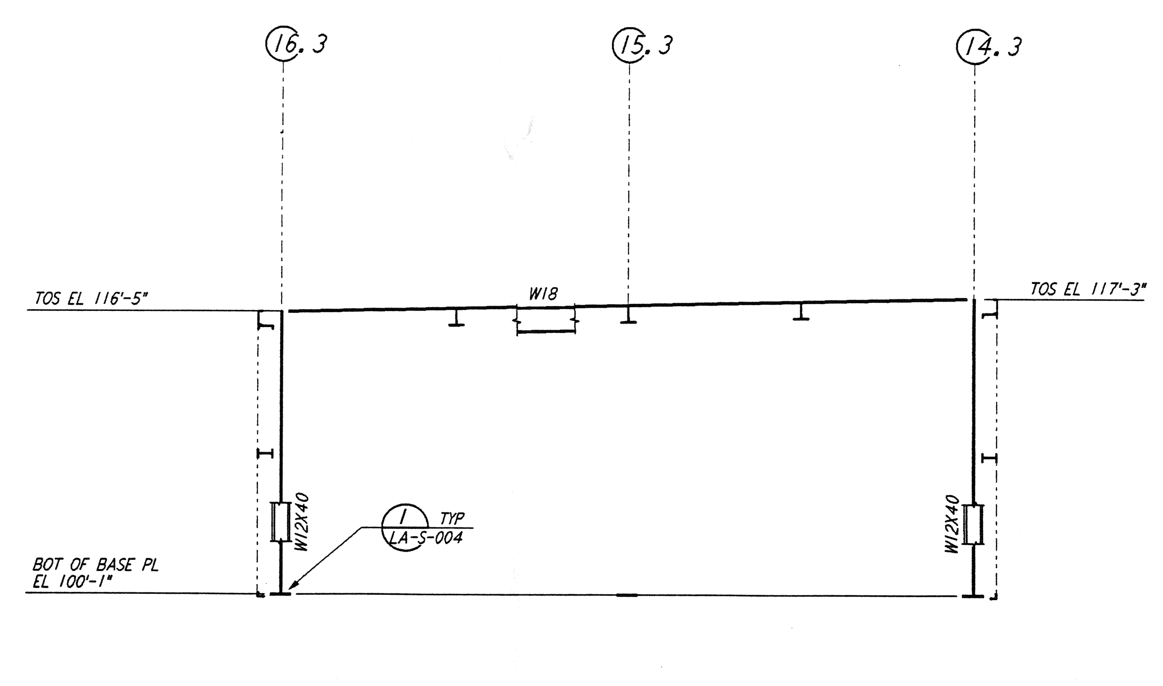
FRAMING ELEVATION AT COLUMN LINE P.3, R, S & T \frac{3}{8}'' = 1'-0''
