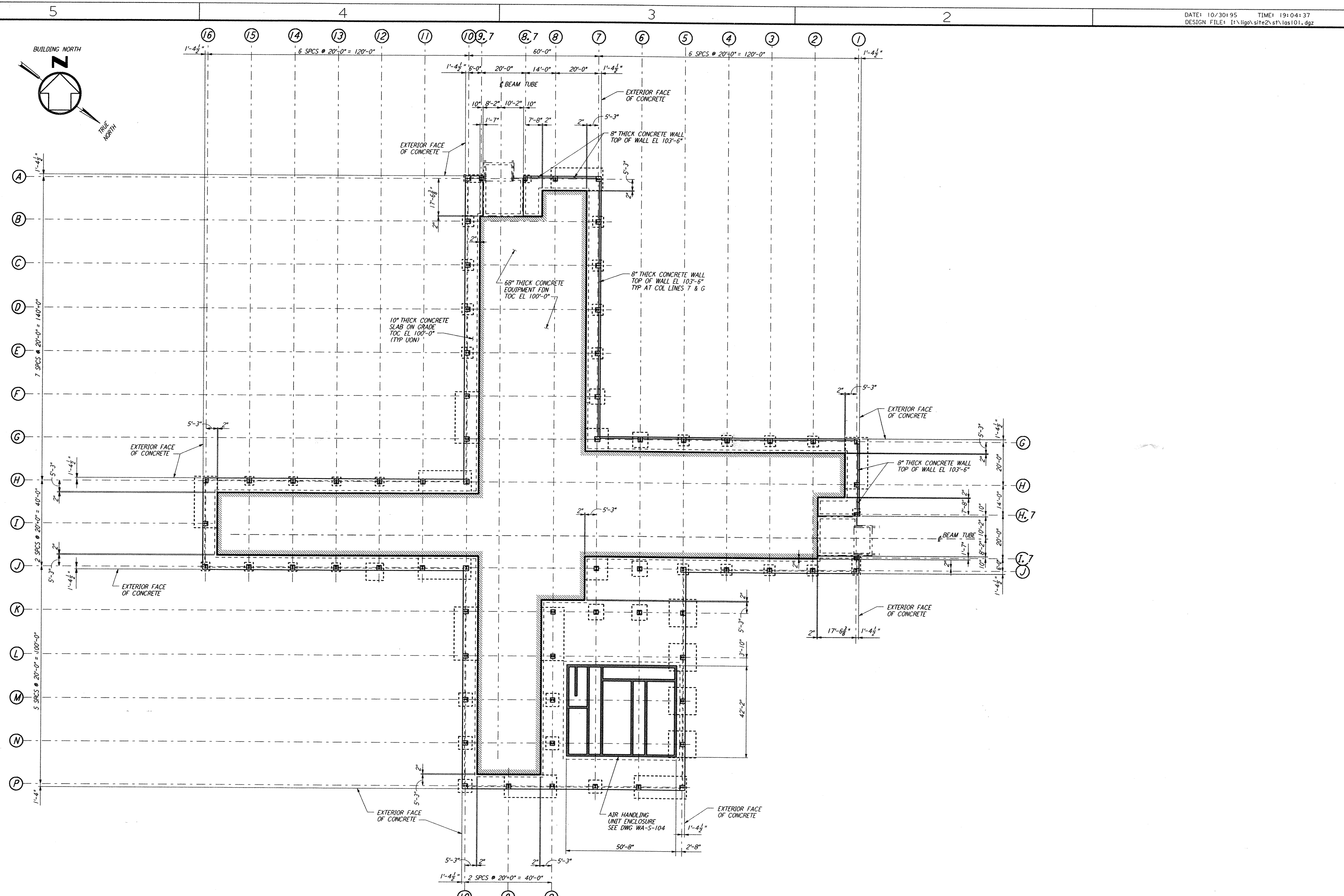
CORNER STATION FOUNDATION PLAN 1/8" = 1'-0"
