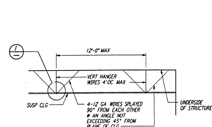
SUSP ACOUSTICAL CLG DET
