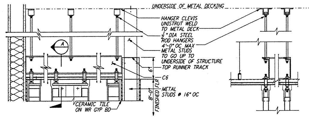
TOILET PARTITION MOUNTING
