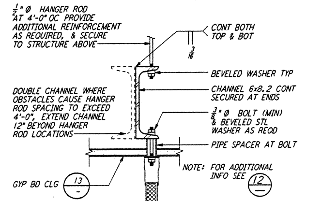
TOILET PARTITION MOUNTING
