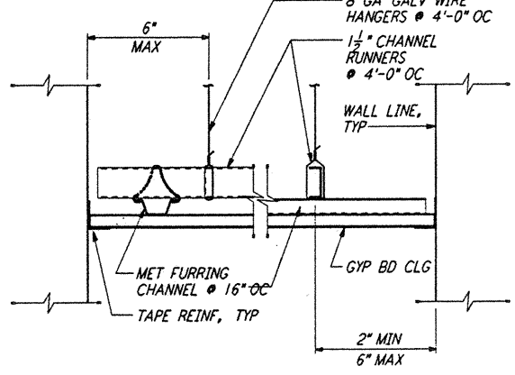
GYPSUM BOARD CEILING
