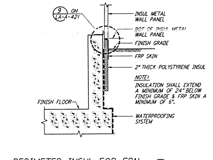
PERIMETER INSUL FOR FDN
