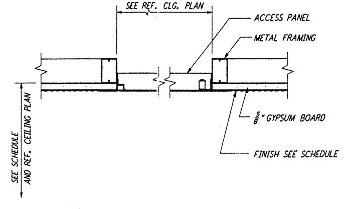
CEILING ACCESS PANEL DET
