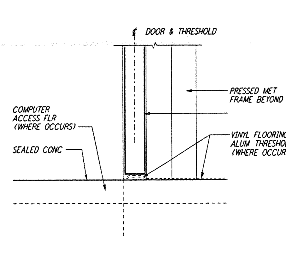
INT THRESHOLD DETAIL
