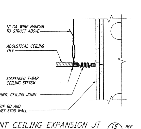
INT CEILING EXPANSION JT
