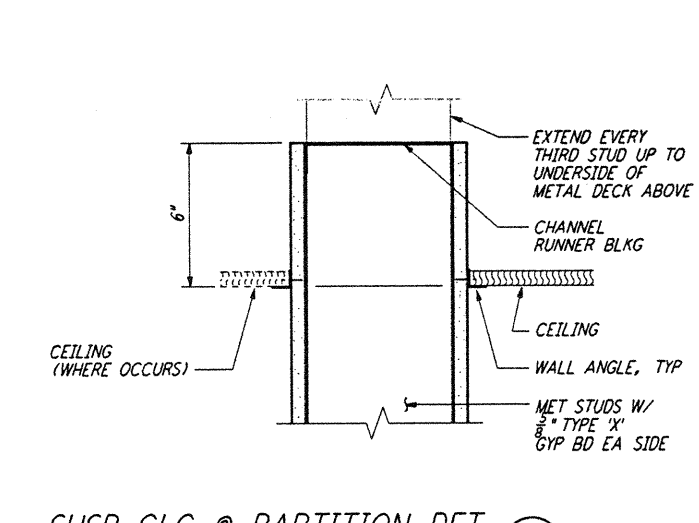
SUSP CLG @ PARTITION DET
