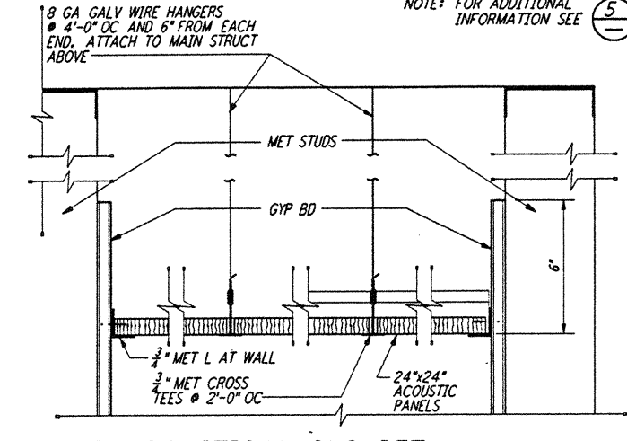
SUSP ACOUSTICAL CLG DET
