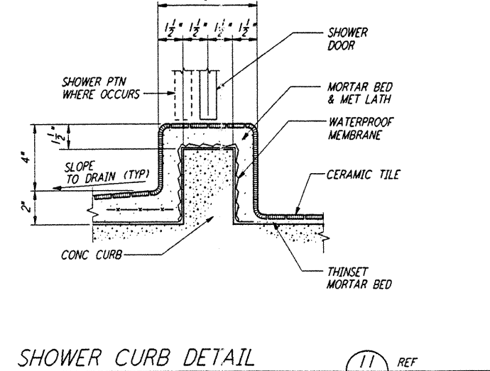
SHOWER CURB DETAIL
