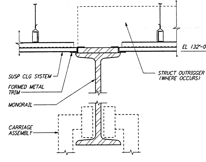
SUSP CLG AT MONORAIL
