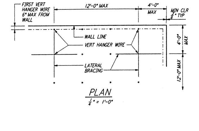
SUSP ACOUSTICAL CLG DET
