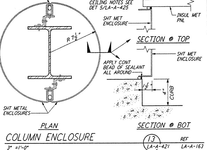
COLUMN ENCLOSURE (13) REF 3'-1'-0" LA-A-421 LA-A-163
