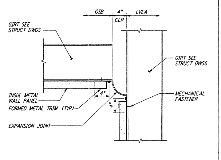
VERT INSIDE CORNER EXP JT (7) REF 1 1/2'-1'-0" LA-A-421 LA-A-132
