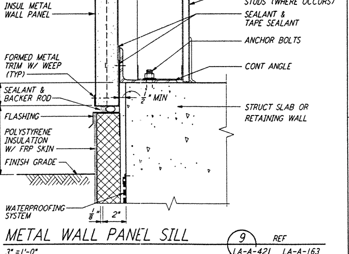
METAL WALL PANEL SILL (9) REF 3'-1'-0" LA-A-421 LA-A-163 LA-A-161
