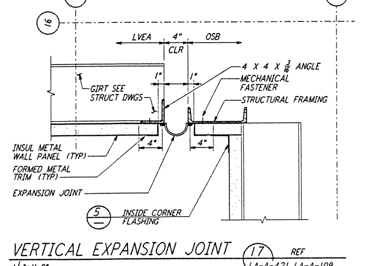
VERTICAL EXPANSION JOINT (17) REF 1 1/2'-1'-0" LA-A-421 LA-A-109
