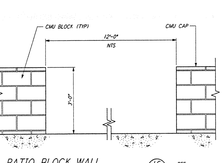
PATIO BLOCK WALL (16) REF 3'-1'-0" LA-A-421 LA-A-108
