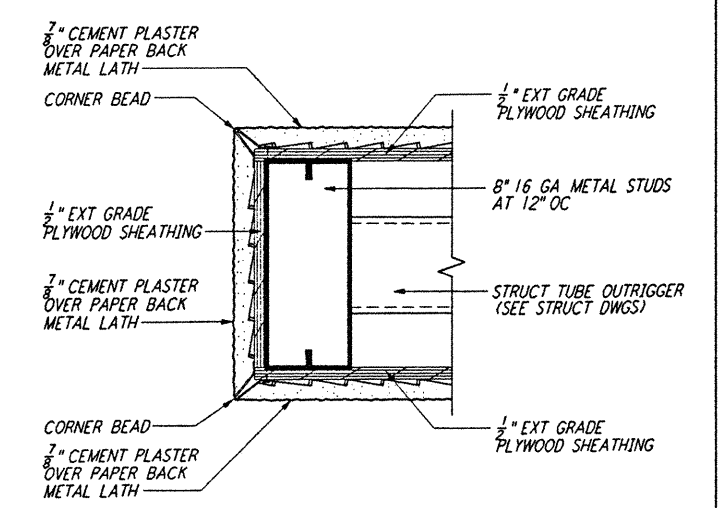
END OF CURVED WALL (10) REF 3'-1'-0" LA-A-421 LA-A-108
