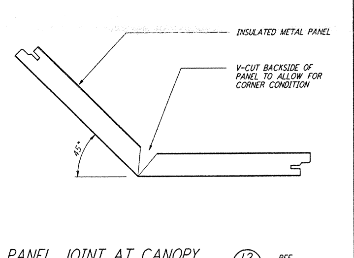
PANEL JOINT AT CANOPY (12) REF 3'-1'-0" LA-A-421 LA-A-132 LA-A-122
