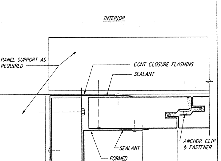
EXP JT @ BM TUBE ENCL (3) REF 3'-1'-0" LA-A-421 LA-A-161
