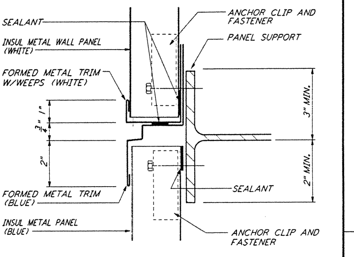
MET WALL PANEL HORIZ JT (2) REF HALF FULL LA-A-421 LA-A-141 LA-A-161
