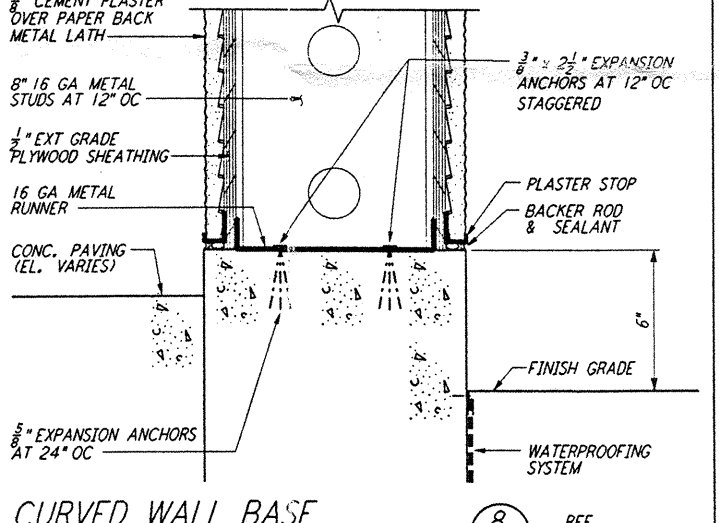
CURVED WALL BASE (8) REF 3'-1'-0" LA-A-421 LA-A-141
