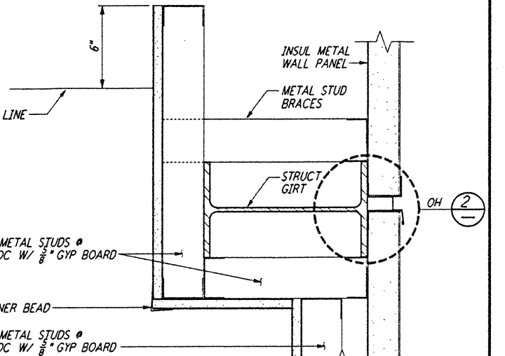
FURRING @ GIRT (1) REF 3'-1'-0" LA-A-421 LA-A-163
