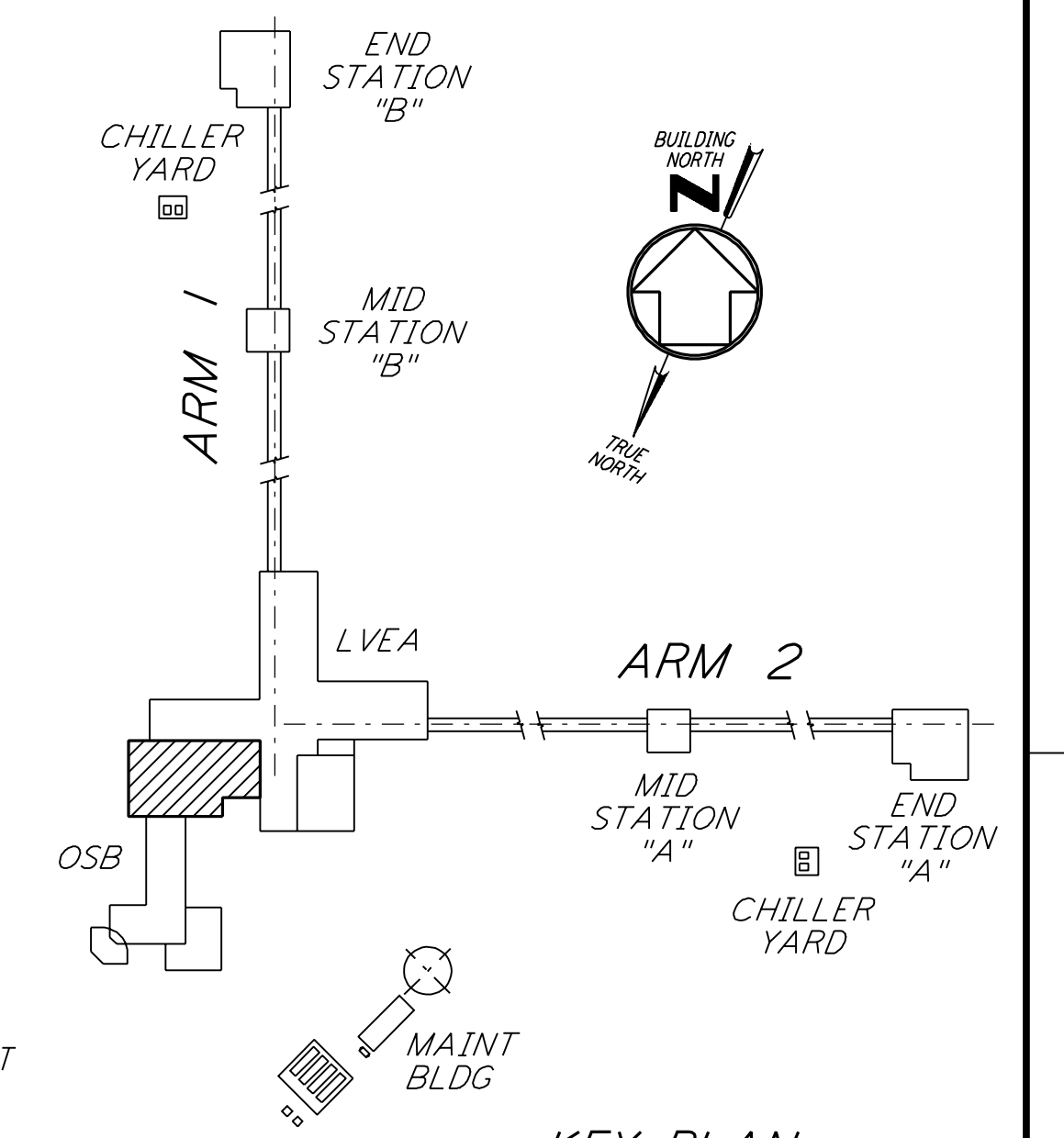
KEY PLAN LIGO-D960880-01-0
