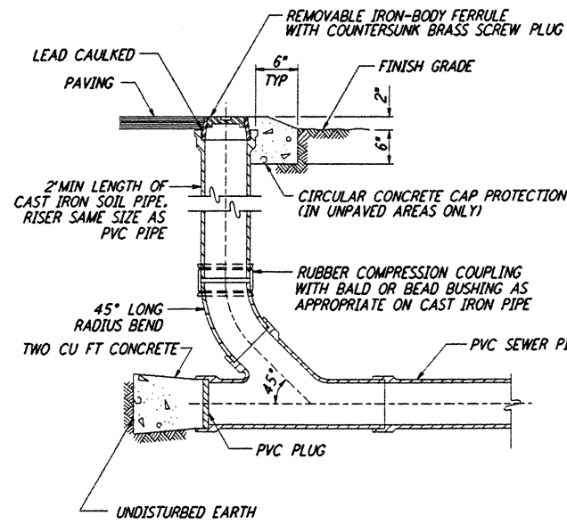
SANITARY SEWER CLEANOUT (2) REF. LA-C-009 LA-C-010 NOT TO SCALE
