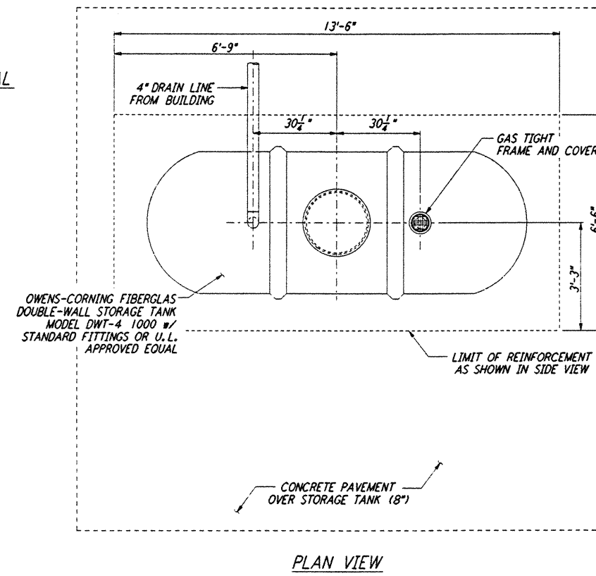
DOUBLE-WALL HOLDING TANK 1000 GALLONS (8) REF. LA-C-009 LA-C-010 NOT TO SCALE
