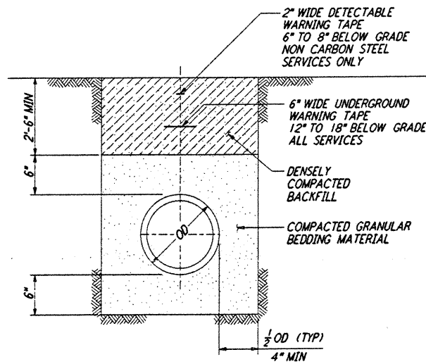
TRENCH BEDDING (5) REF. LA-C-009 LA-C-010 LA-C-027 LA-C-047 NOT TO SCALE
