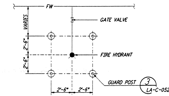
GUARD POST LOCATIONS (6) REF. LA-C-009 LA-C-010 NOT TO SCALE
