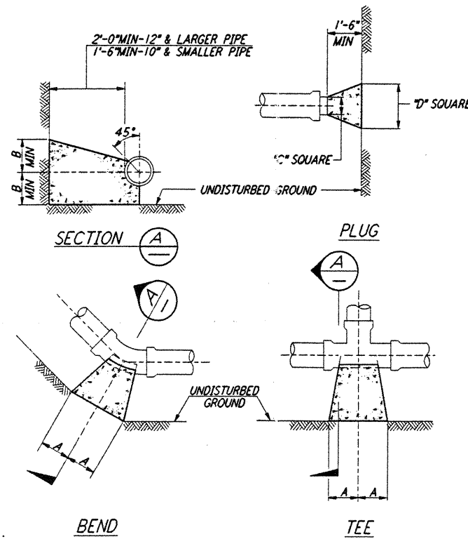
THRUST BLOCK (3) REF. LA-C-009 LA-C-010 NOT TO SCALE
