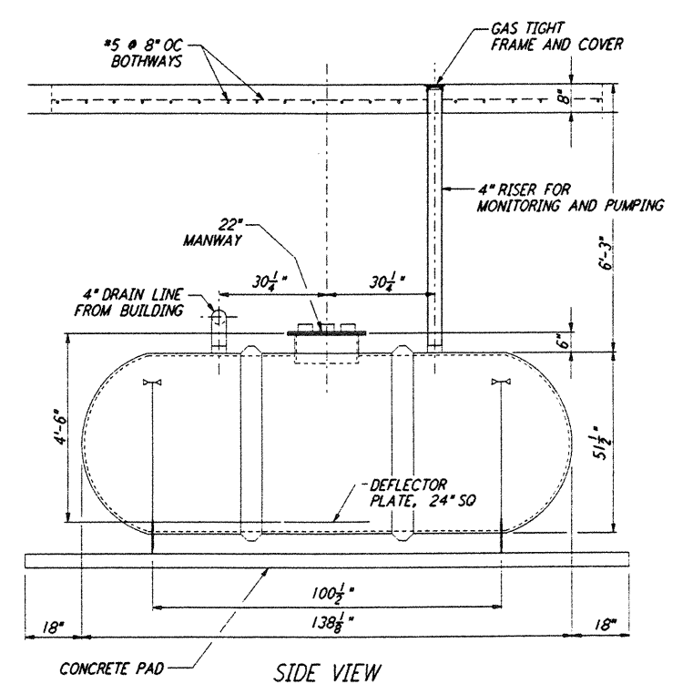
SIDE VIEW
