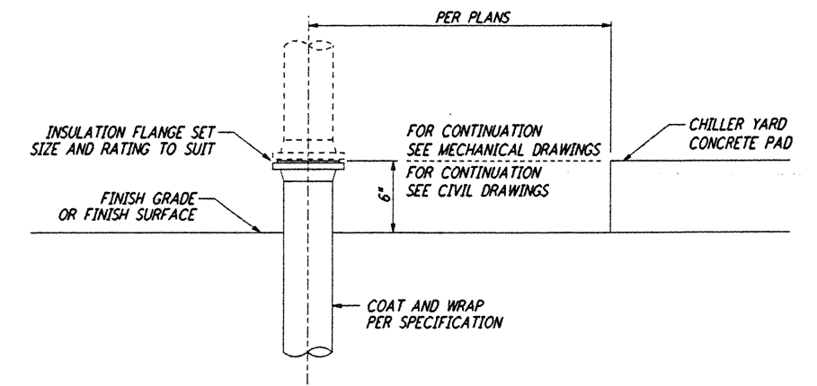
PIPE CONNECTION (4) REF. LA-C-009 LA-C-010 LA-C-027 LA-C-047 NOT TO SCALE
