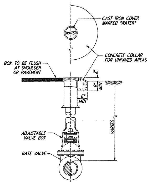
VALVE BOX (1) REF. LA-C-009 LA-C-010 NOT TO SCALE NOTE: VALVE SIZE 12" MAXIMUM
