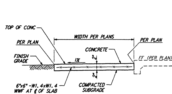
CONCRETE WALKWAY (1) REF LA-C-005 LA-C-006 LA-C-007 LA-C-008 NOT TO SCALE
