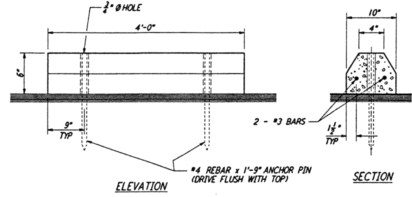
CONCRETE PARKING BUMPER (4) REF LA-C-005 LA-C-006 LA-C-021 LA-C-025 LA-C-041 LA-C-045 NOT TO SCALE
