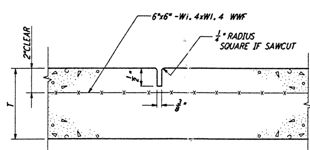
CONTRACTION JOINT (7) REF LA-C-005 LA-C-006 LA-C-021 LA-C-025 LA-C-041 LA-C-045 NOT TO SCALE (CO) (SPACING: 20' MAX)
