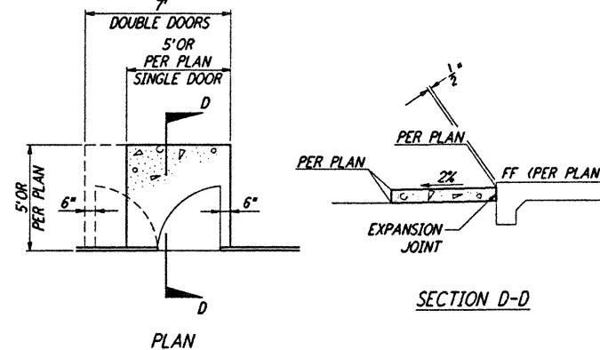
CONCRETE STOOP (2) REF LA-C-005 LA-C-006 LA-C-025 LA-C-045 NOT TO SCALE
