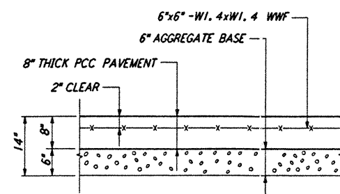
CONCRETE PAVEMENT (3) REF LA-C-005 LA-C-006 LA-C-021 LA-C-025 LA-C-041 LA-C-045 NOT TO SCALE
