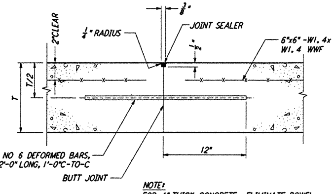
CONSTRUCTION JOINT (6) REF LA-C-005 LA-C-006 LA-C-021 LA-C-025 LA-C-041 LA-C-045 NOT TO SCALE (CJ) (SEPARATE POURS OR END OF DAY)
