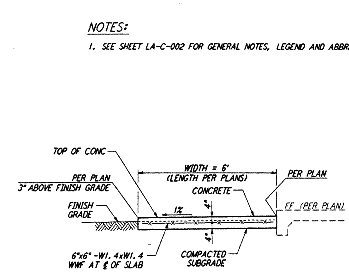
RAISED CONCRETE PAD FOR ELECTRICAL TRANSFORMERS (9) REF LA-C-051 LA-C-005 NOT TO SCALE
