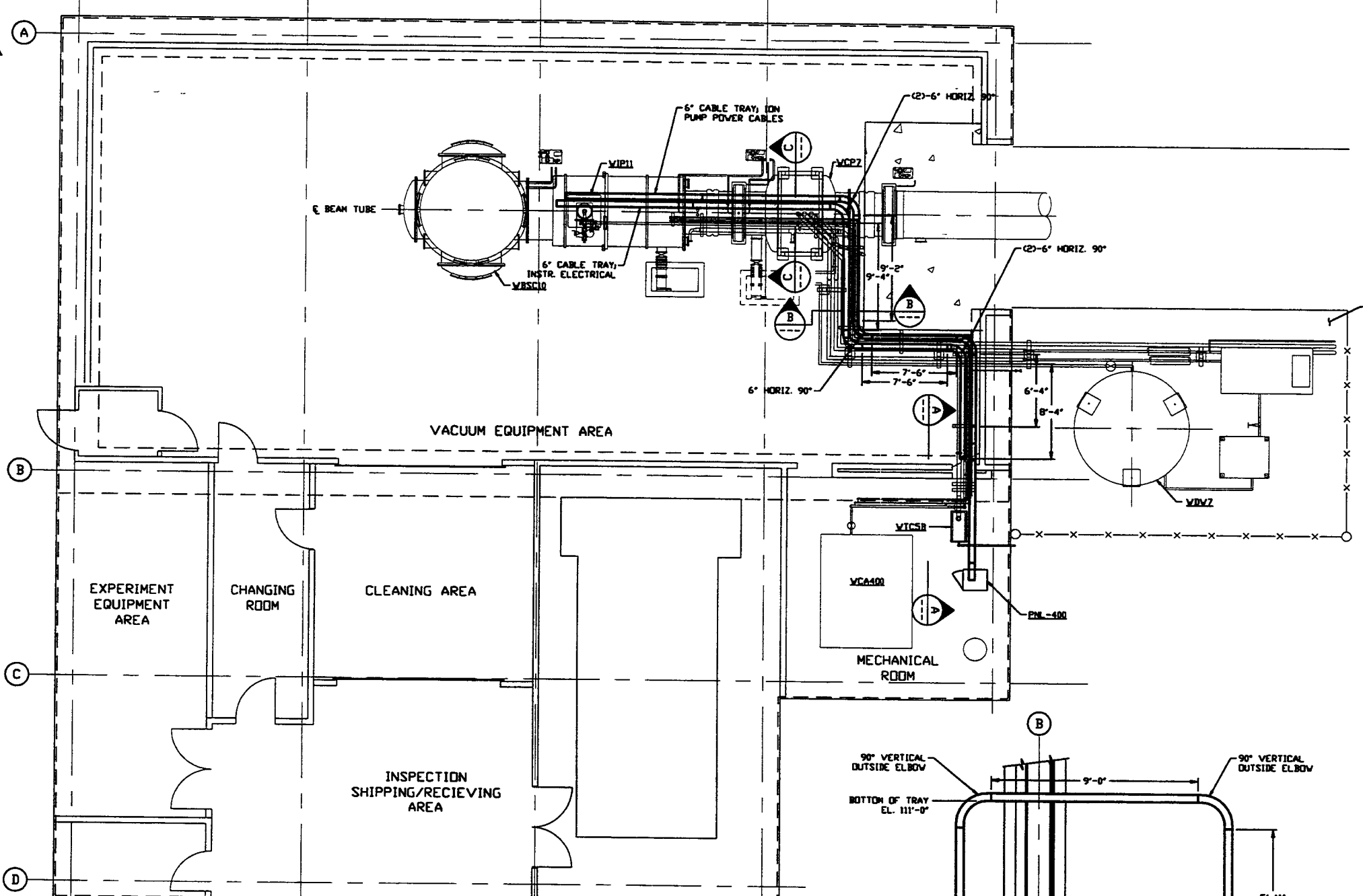
LEFT END STATION PLAN @ EL. 100'-0"
