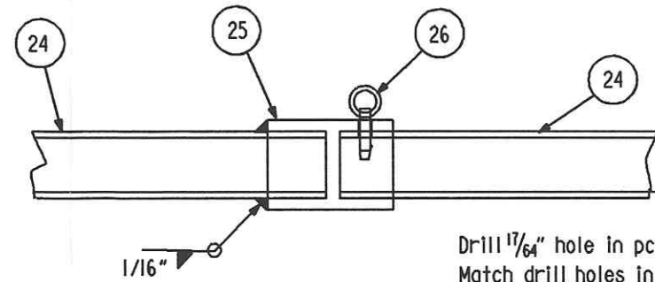
Push Pipe Assemblies (typical six places)
