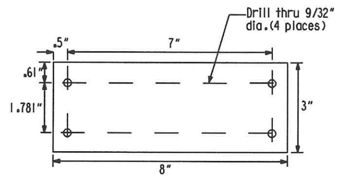
Pc. 10 Make from 1/4" thk. 304 ss plate
