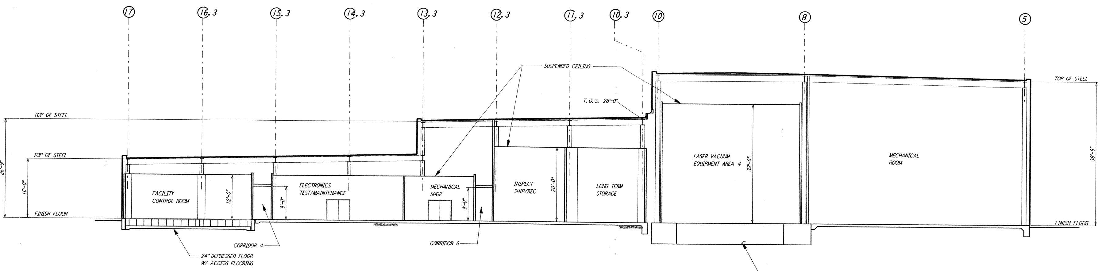
SECTION B \frac{1}{8}'' = 1'-0'' WA-A-107
