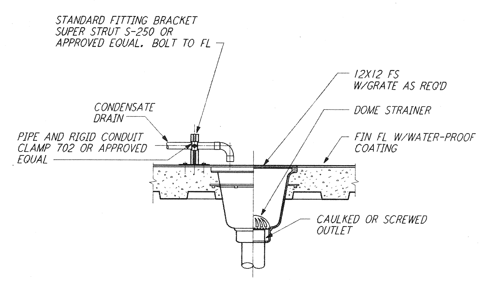
FLOOR SINK DETAIL 3 REF NTS WA-P-411
