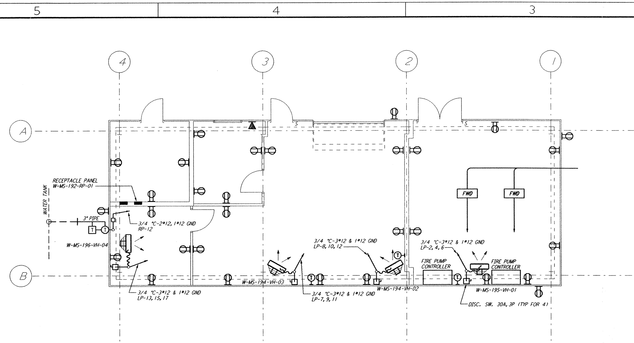
MAINTENANCE BUILDING FLOOR PLAN \frac{1}{4}'' = 1'-0''
