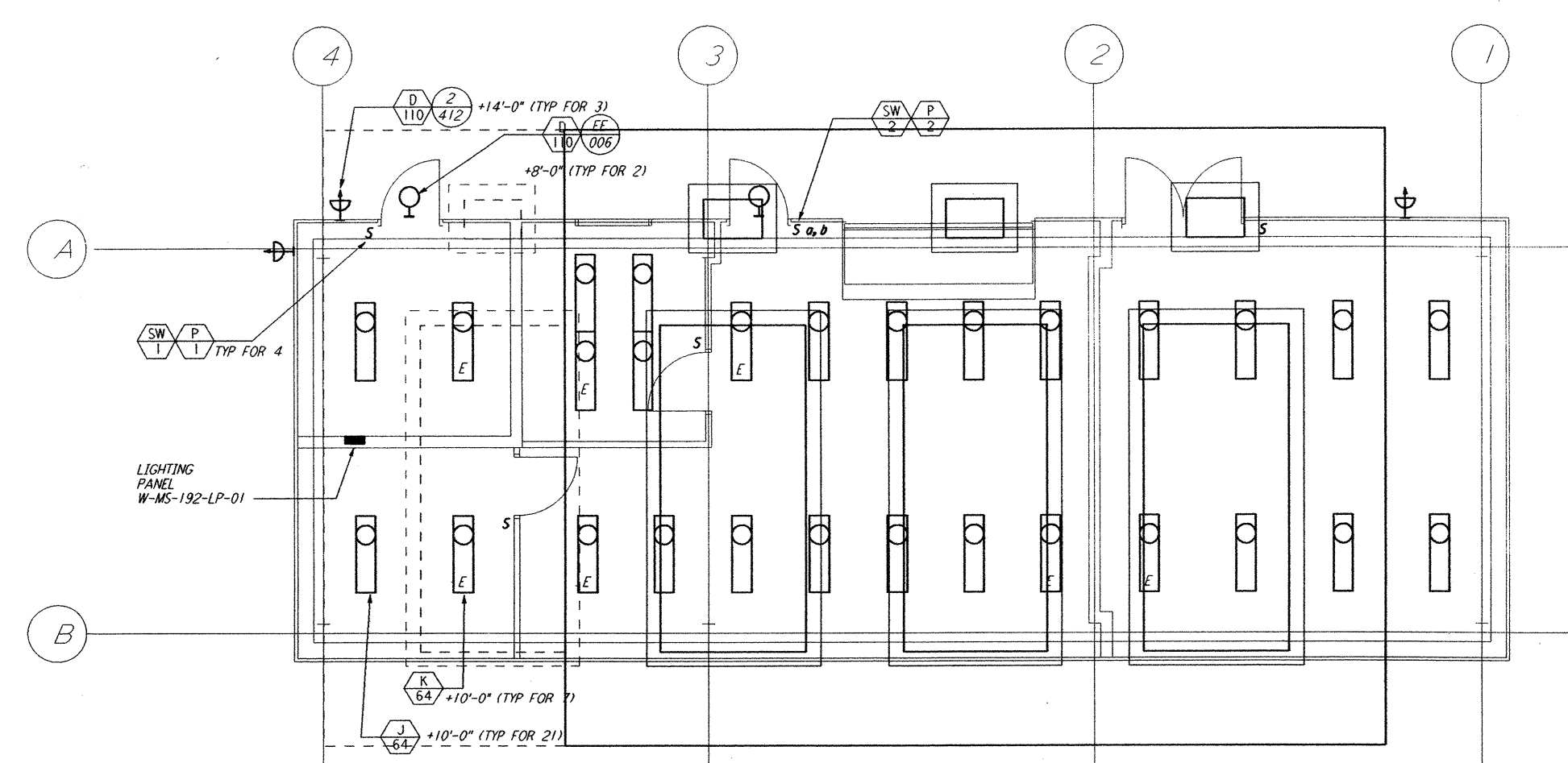
MAINTENANCE BUILDING FLOOR PLAN \frac{1}{4}'' = 1'-0''
