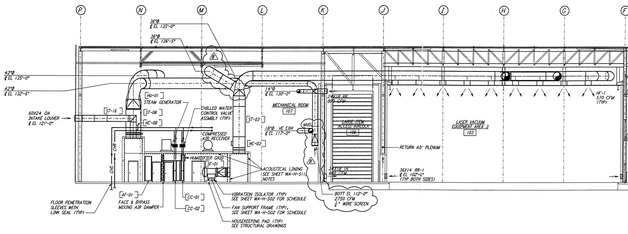
SECTION B REF \frac{1}{8}'' = 1'-0'' WA-H-552 WA-H-511
