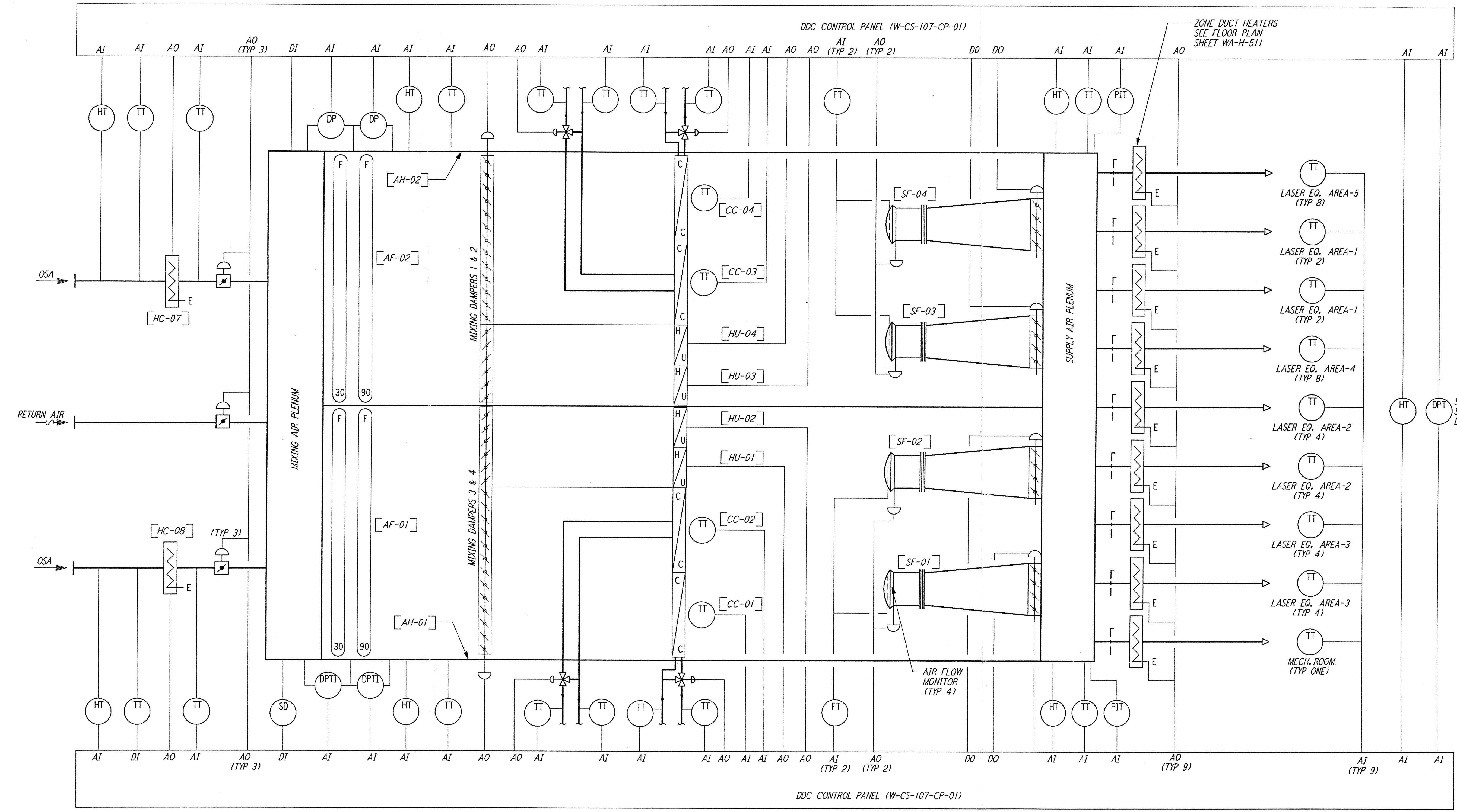
LVEA AIR FLOW & CONTROL DIAGRAM (AH-01 & AH-02)
