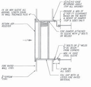
WALL MOUNTED FIRE DAMPER (1) REF NTS WA-H-411
