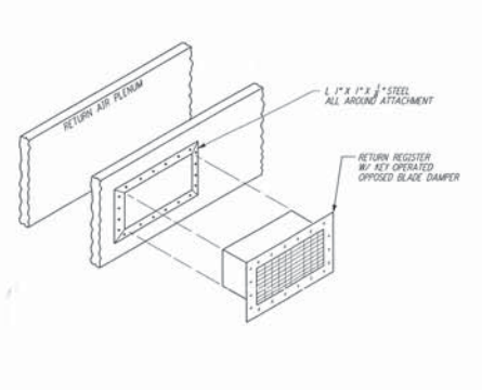
REGISTER MOUNTING DETAIL (8) REF NTS WA-H-411
