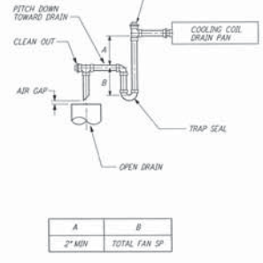
CONDENSATE DRAIN DETAIL (10) REF NTS WA-H-411
