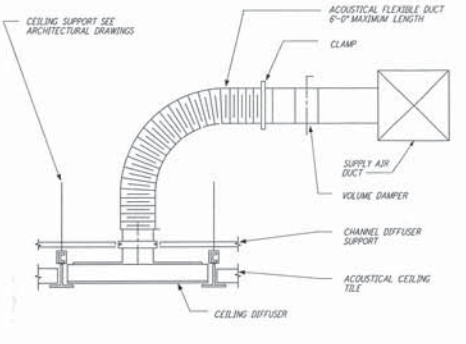
FLEXIBLE DUCT CONNECTION (4) REF NTS WA-H-411
