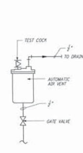
AUTOMATIC AIR VENT (11) REF NTS WA-H-411
