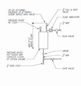
CHEMICAL FEEDER DETAIL (7) REF NTS WA-H-411
