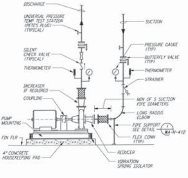
PUMP CONNECTION DETAIL (5) REF NTS WA-H-411
