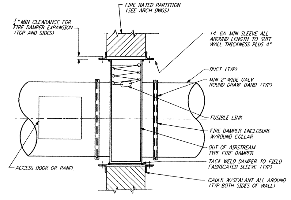
ROUND DUCT FIRE DAMPER MOUNTING DETAIL (3) REF NTS WA-H-411 XXXXXXXX
