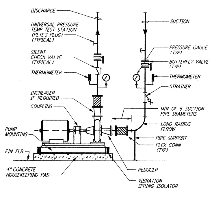
PUMP CONNECTION DETAIL (5) REF NTS WA-H-411 XXXXXXXX
