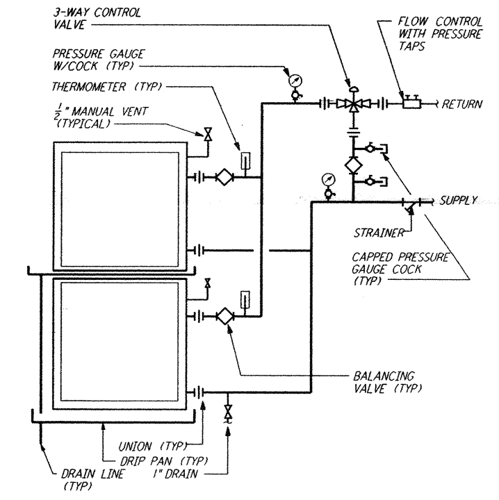
MULTIPLE COIL PIPING DETAIL (6) REF NTS WA-H-411 XXXXXXXX
