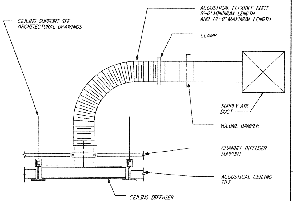
FLEXIBLE DUCT CONNECTION (4) REF NTS WA-H-411 XXXXXXXX
