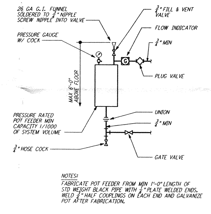
CHEMICAL FEEDER DETAIL (7) REF NTS WA-H-411 XXXXXXXX
