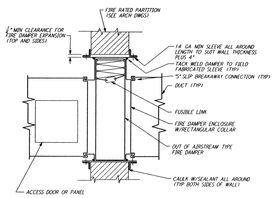
RECTANGULAR DUCT FIRE DAMPER (2) REF NTS WA-H-411 XXXXXXXX
