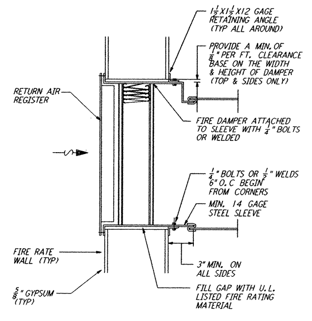
WALL MOUNTED FIRE DAMPER (1) REF NTS WA-H-411 XXXXXXXX
