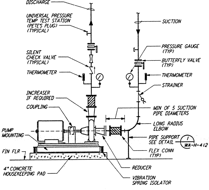
PUMP CONNECTION DETAIL (5) REF NTS WA-H-411
