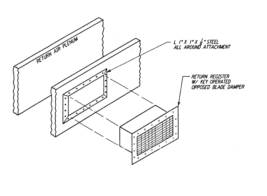
REGISTER MOUNTING DETAIL (8) REF NTS WA-H-411
