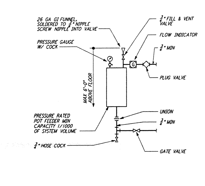
CHEMICAL FEEDER DETAIL (7) REF NTS WA-H-411
