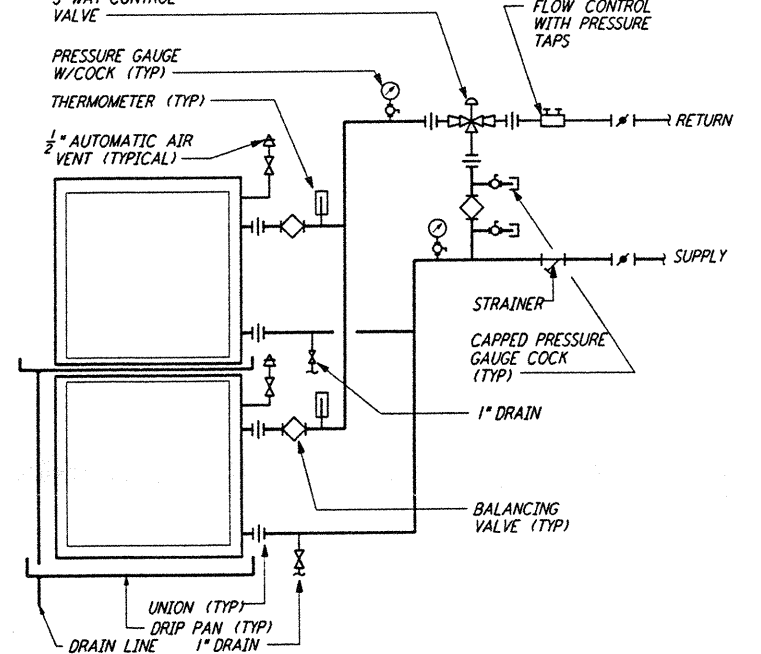
MULTIPLE COIL PIPING DETAIL (6) REF NTS WA-H-411
