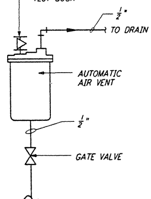
AUTOMATIC AIR VENT (11) REF NTS WA-H-411
