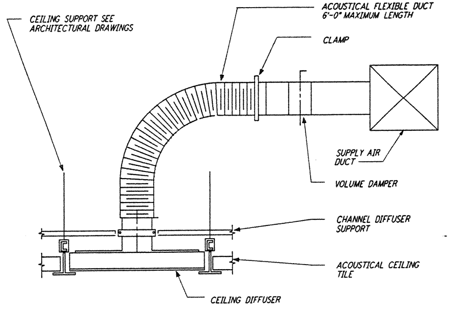
FLEXIBLE DUCT CONNECTION (4) REF NTS WA-H-411
