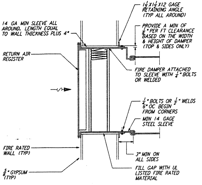
WALL MOUNTED FIRE DAMPER (1) REF NTS WA-H-411
