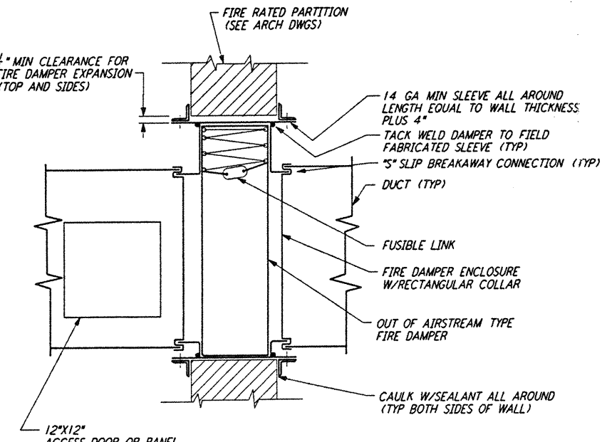
RECTANGULAR DUCT FIRE DAMPER (2) REF NTS WA-H-411
