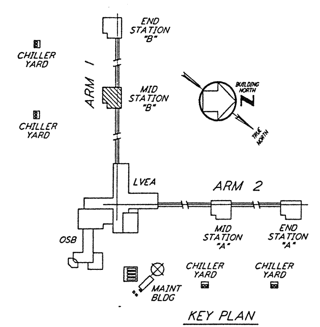
KEY PLAN 1/4" = 1'-0"
