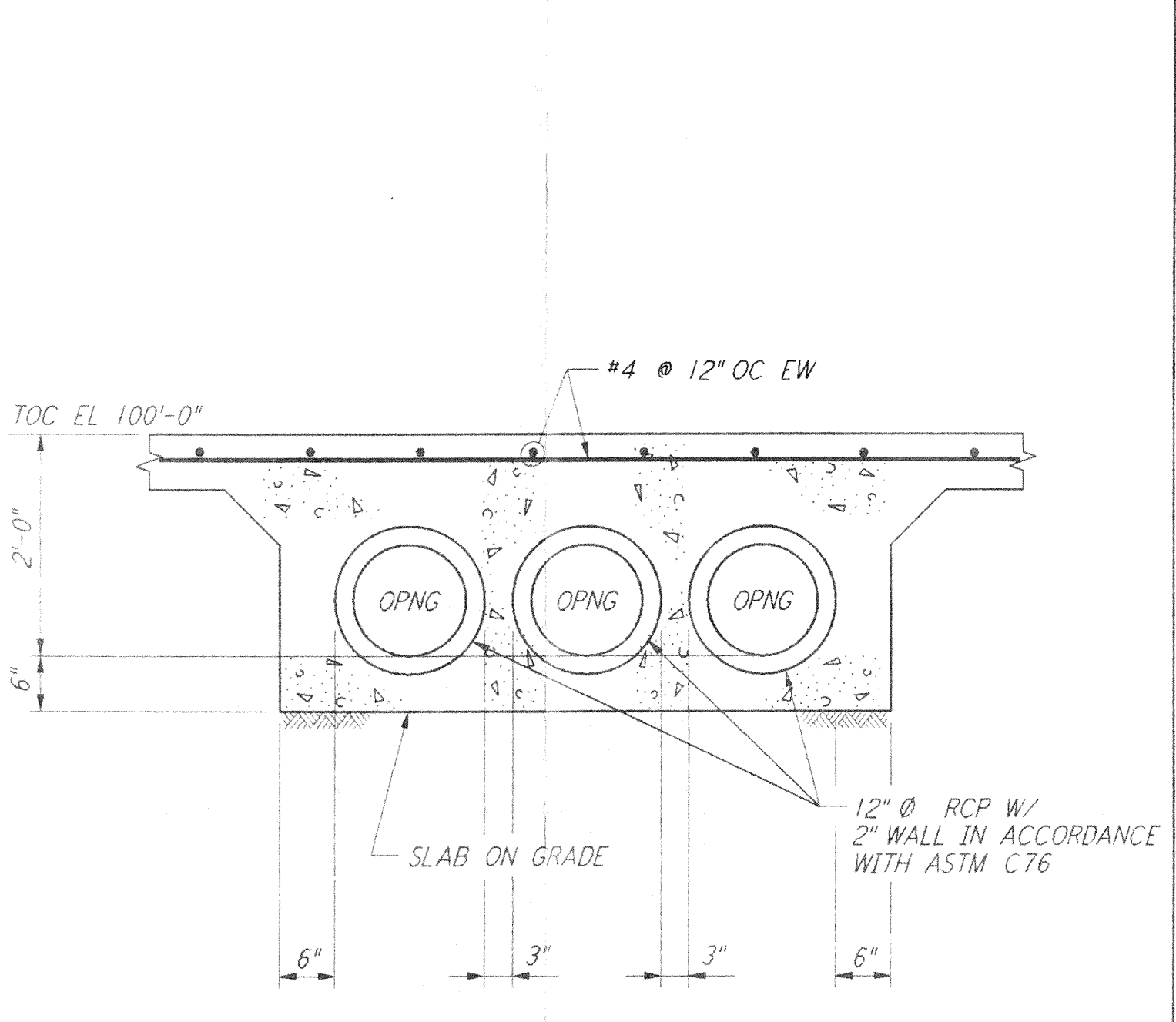
SECTION H REF \frac{3}{4}'' = 1'-0'' WA-S-405 WA-S-102
