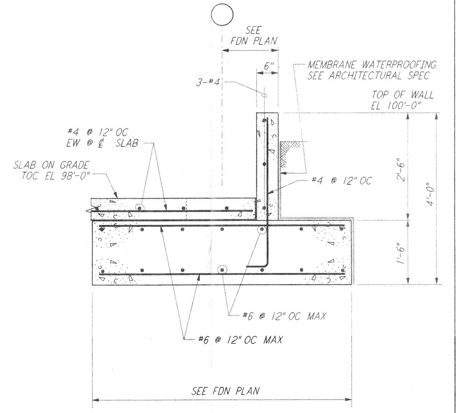
SECTION N REF \frac{3}{4}'' = 1'-0'' WA-S-405 WA-S-102
