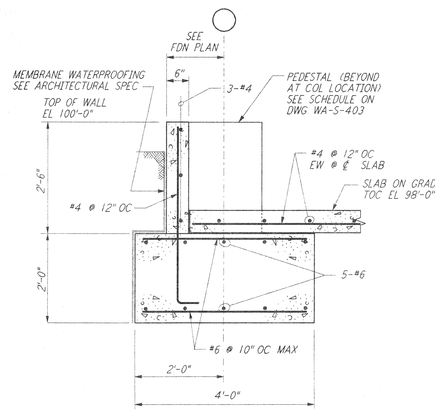
SECTION A REF \frac{3}{4}'' = 1'-0'' WA-S-405 WA-S-102
