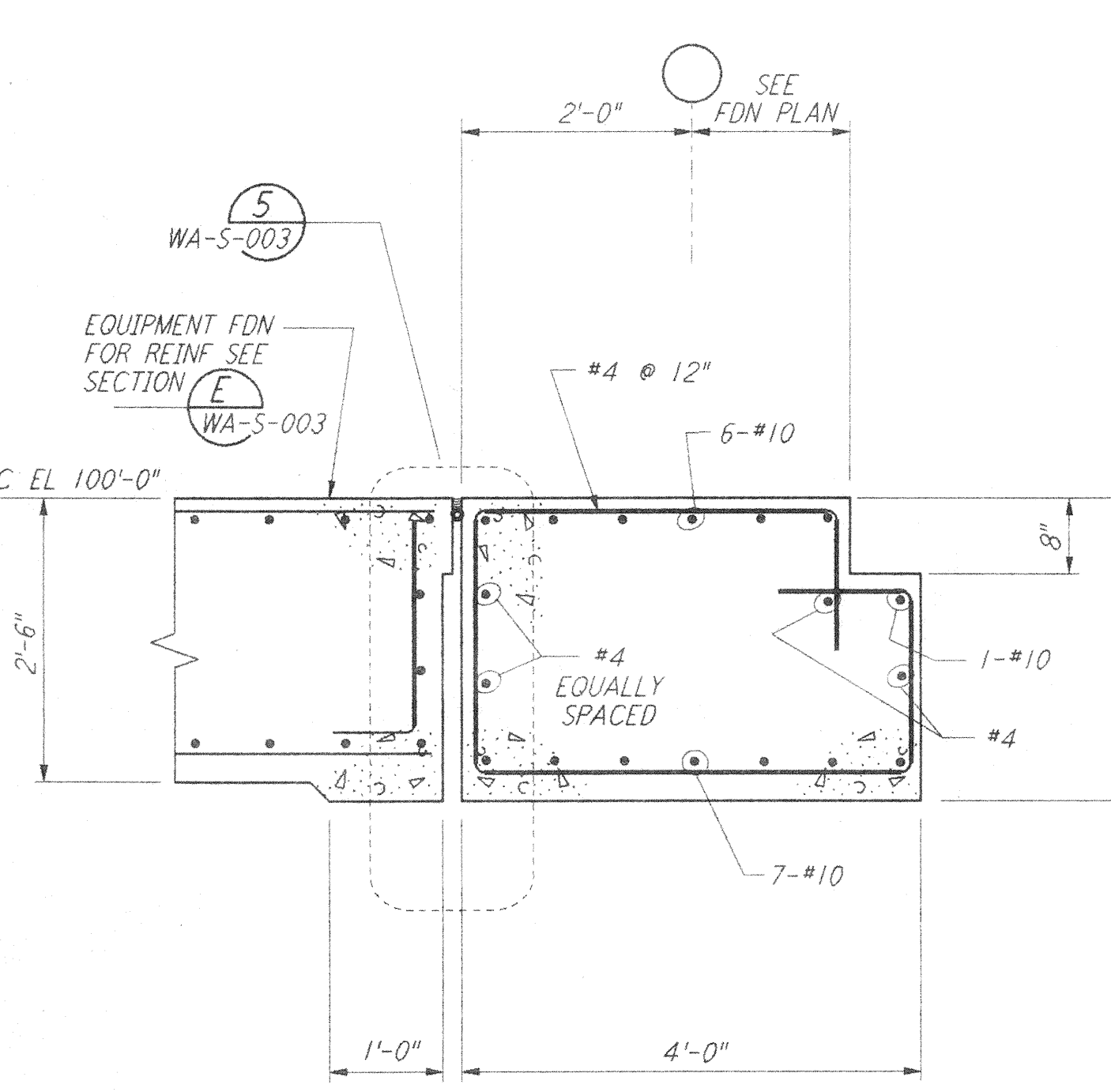
SECTION L REF \frac{3}{4}'' = 1'-0'' WA-S-405 WA-S-501
