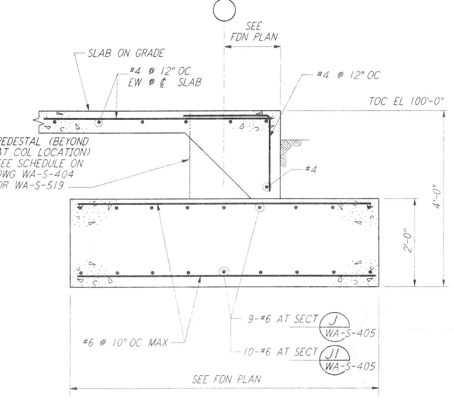
SECTION J, J1 REF \frac{3}{4}'' = 1'-0'' WA-S-405 WA-S-501
