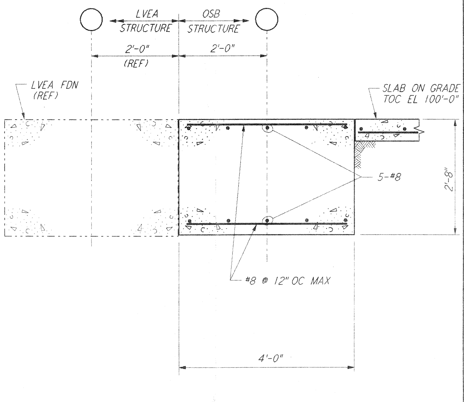
SECTION C REF \frac{3}{4}'' = 1'-0'' WA-S-405 WA-S-102
