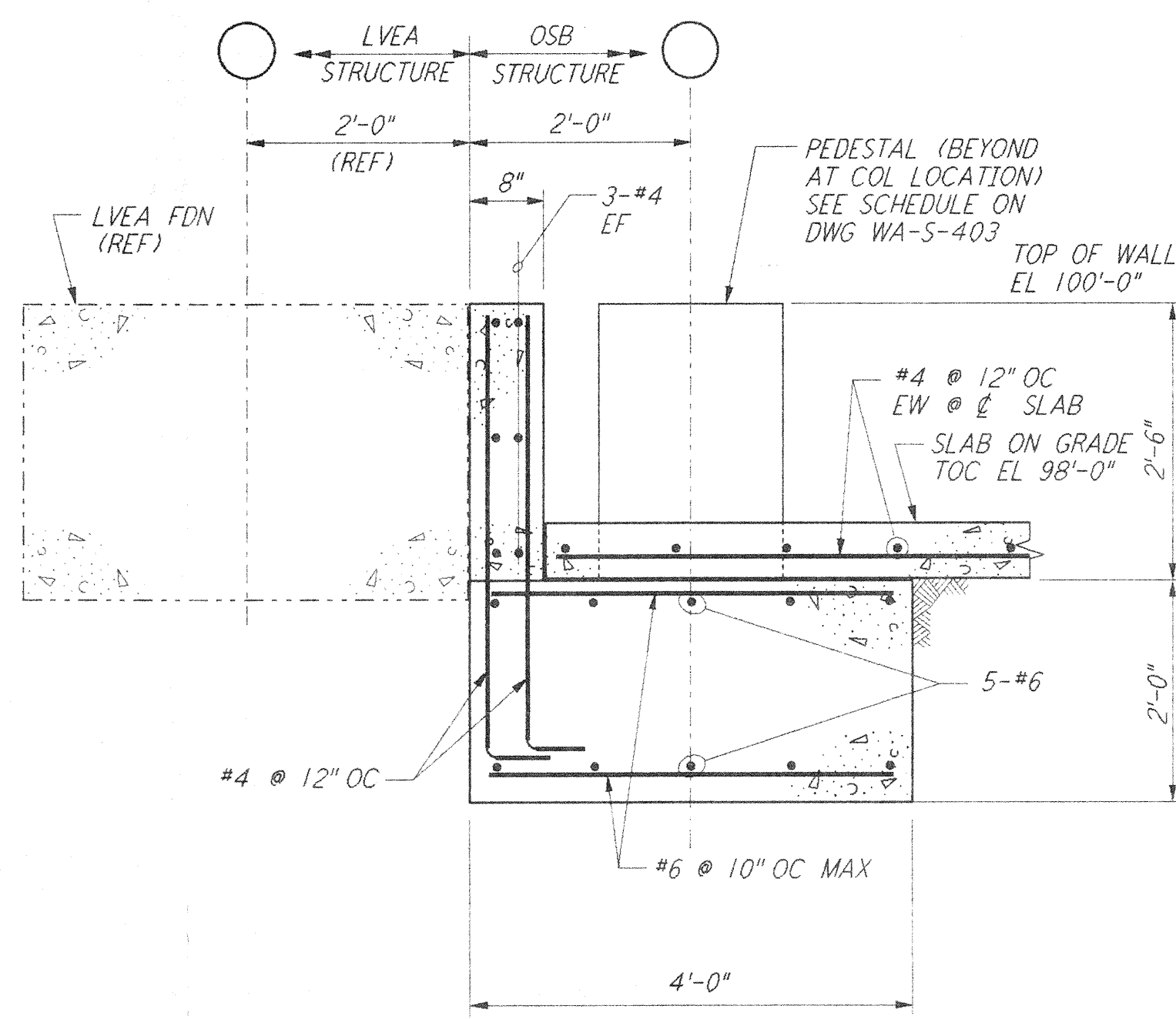
SECTION B REF \frac{3}{4}'' = 1'-0'' WA-S-405 WA-S-102
