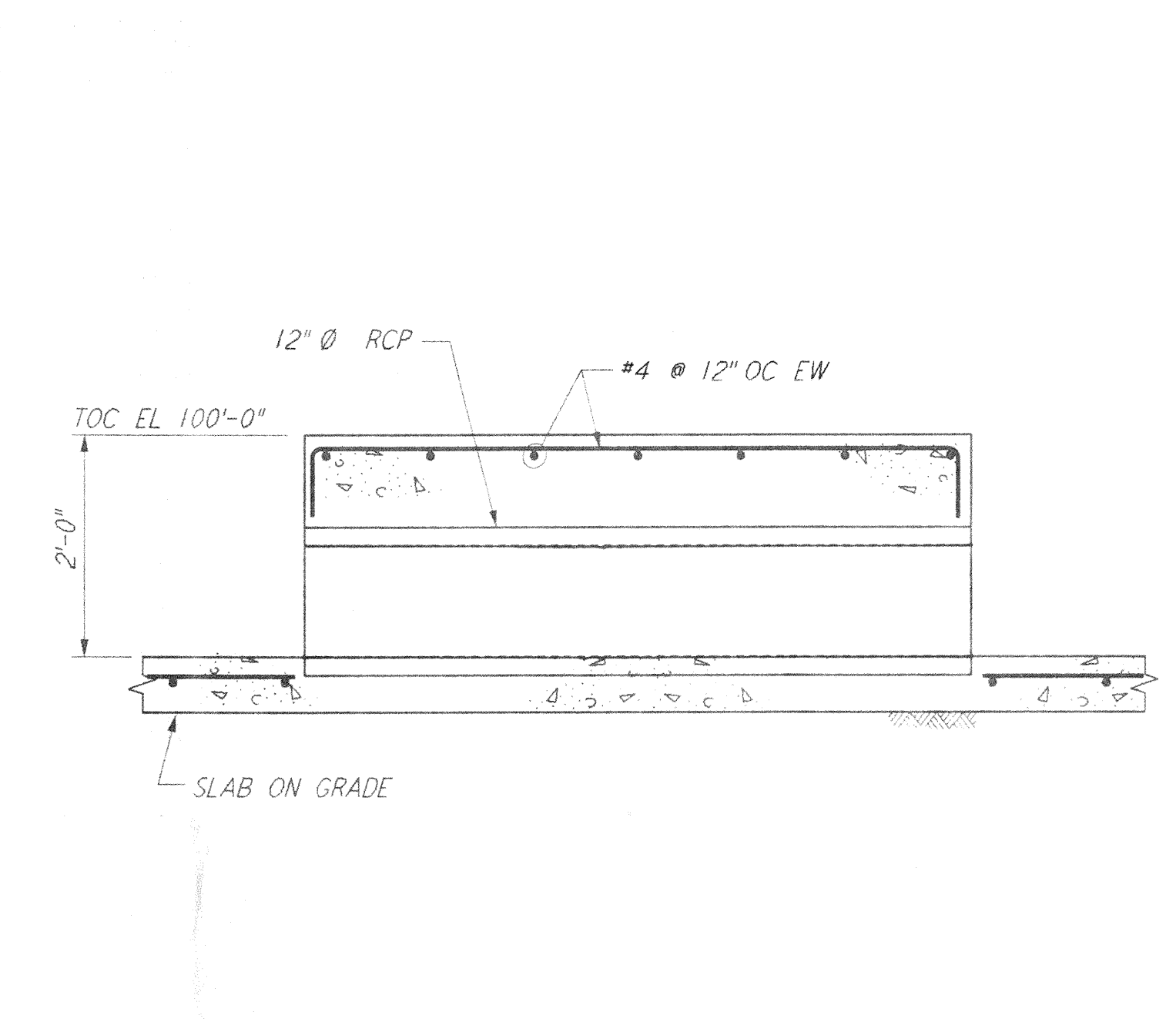
SECTION G REF \frac{3}{4}'' = 1'-0'' WA-S-405 WA-S-102
