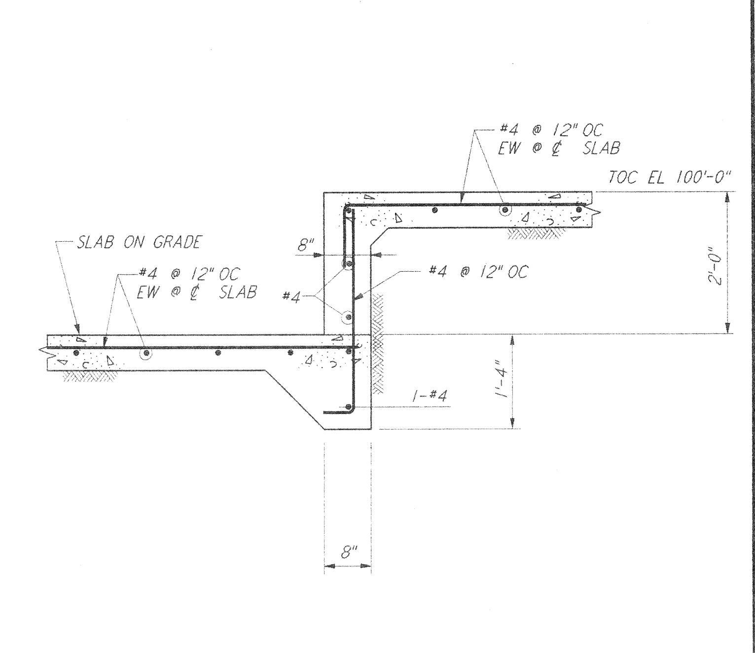
SECTION E REF \frac{3}{4}'' = 1'-0'' WA-S-405 WA-S-102
