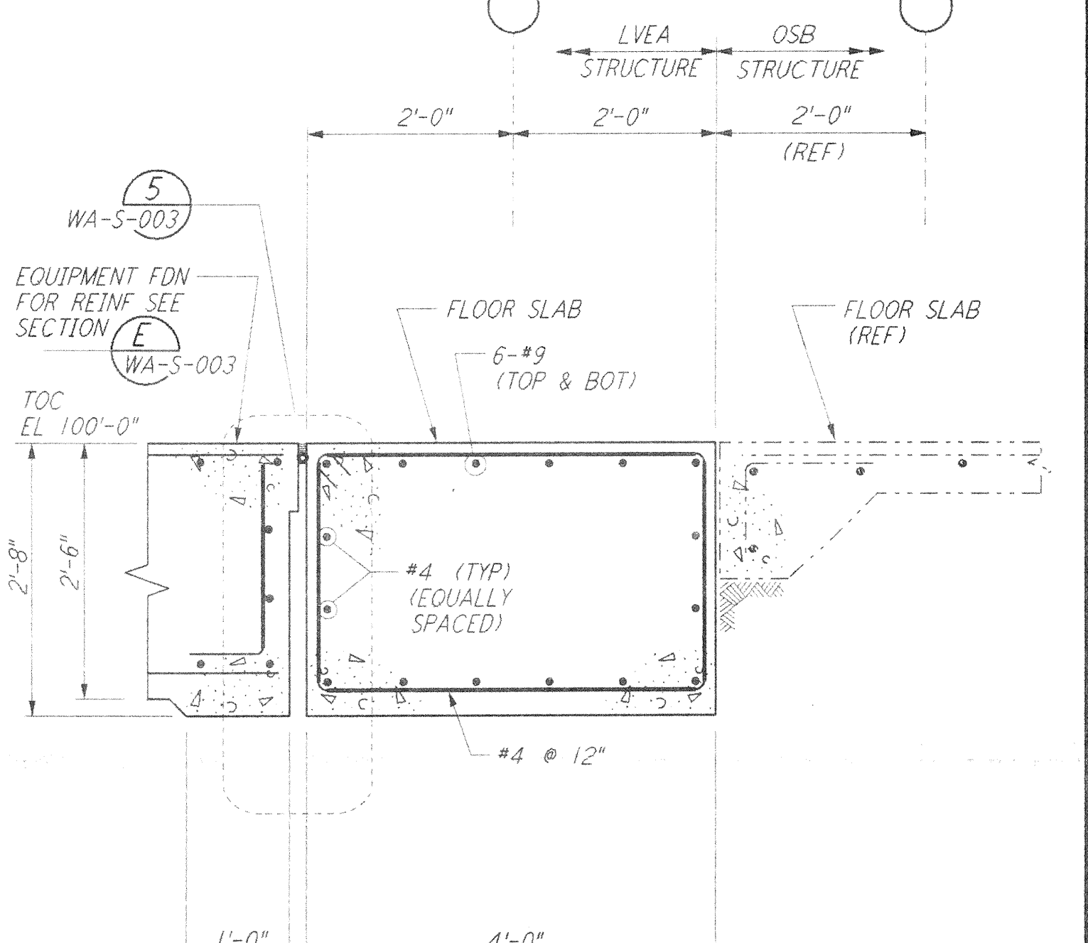
SECTION K REF \frac{3}{4}'' = 1'-0'' WA-S-405 WA-S-501
