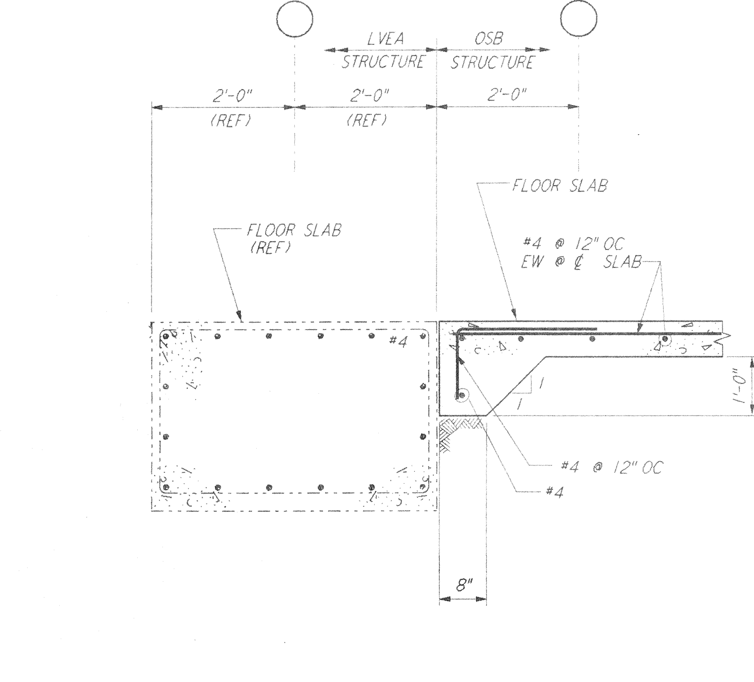
SECTION M REF \frac{3}{4}'' = 1'-0'' WA-S-405 WA-S-102
