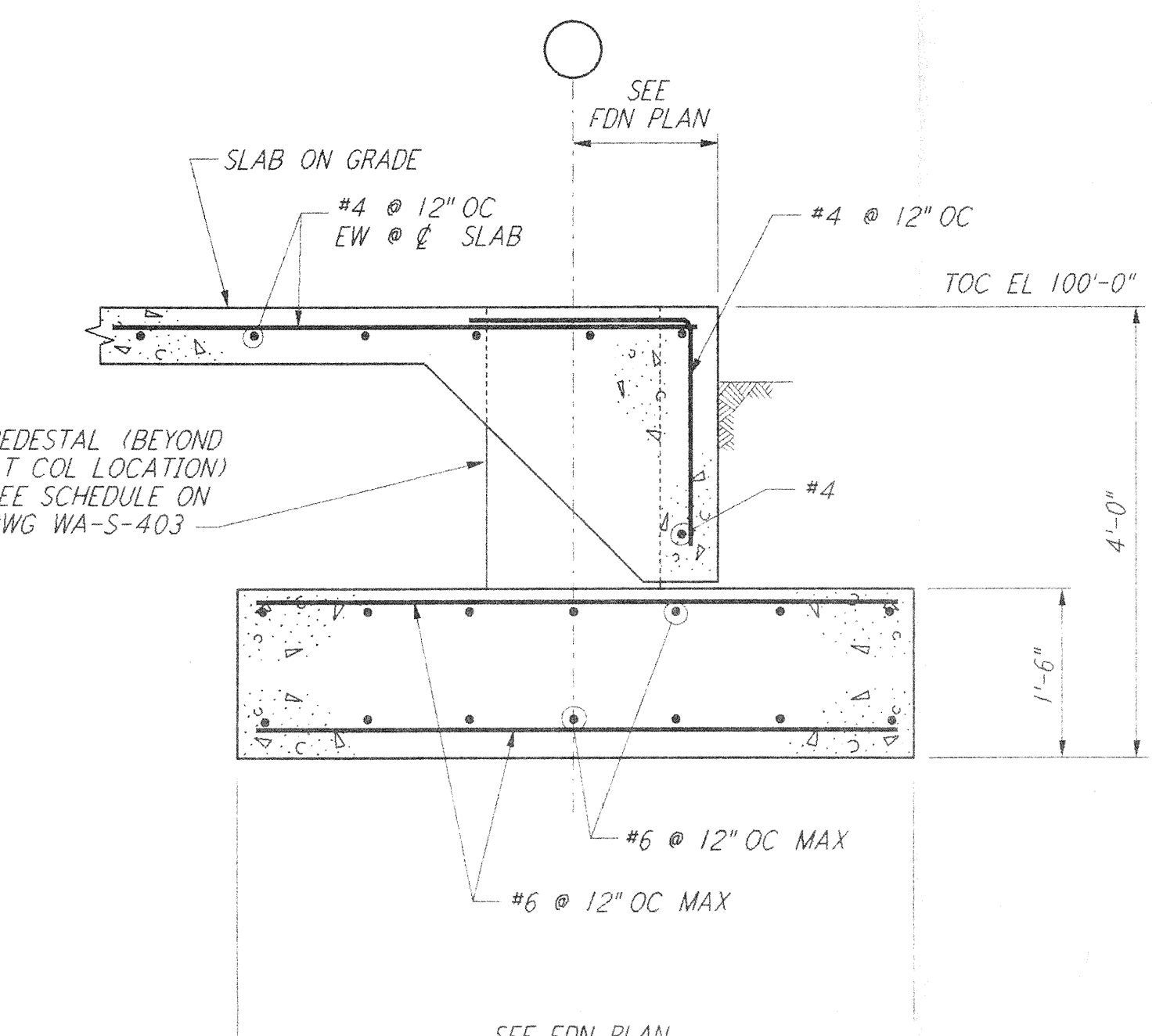
SECTION D REF \frac{3}{4}'' = 1'-0'' WA-S-405 WA-S-102
