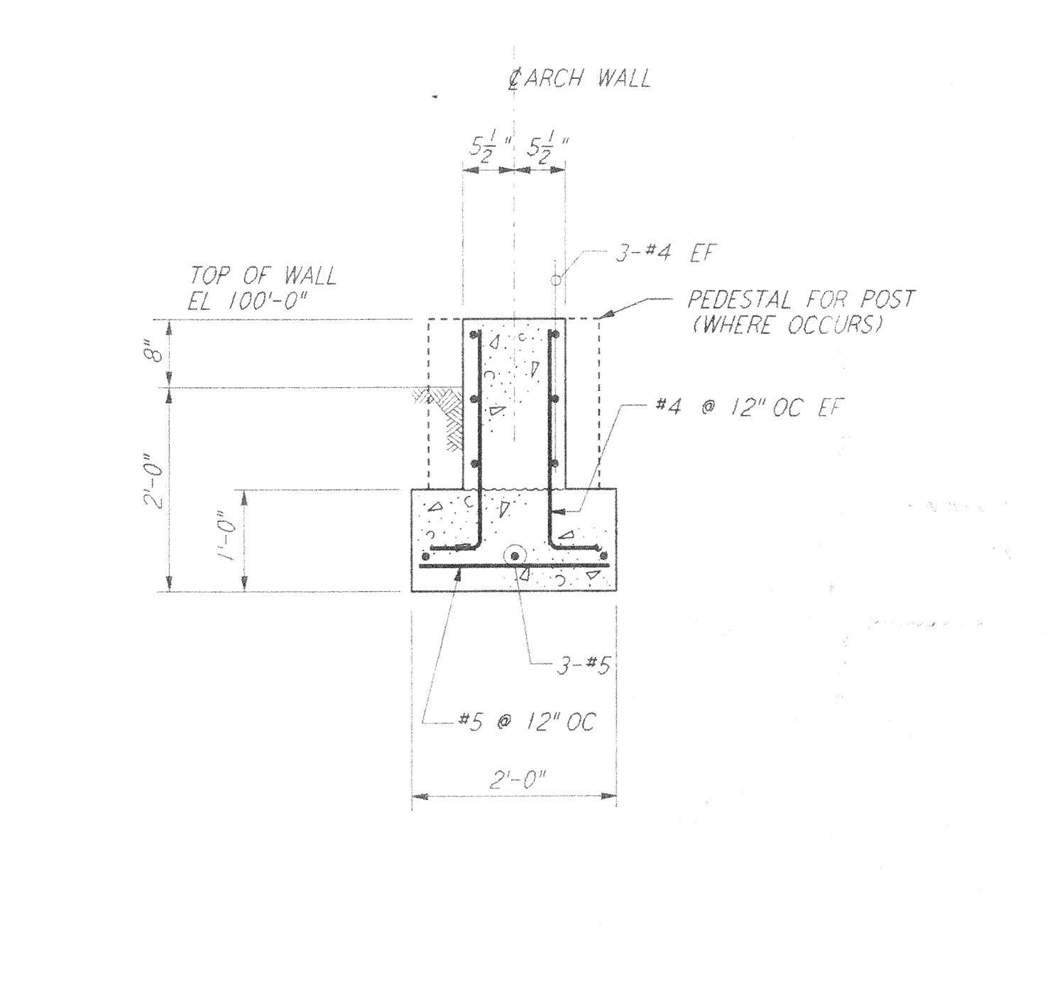
SECTION P REF \frac{3}{4}'' = 1'-0'' WA-S-405 WA-S-102
