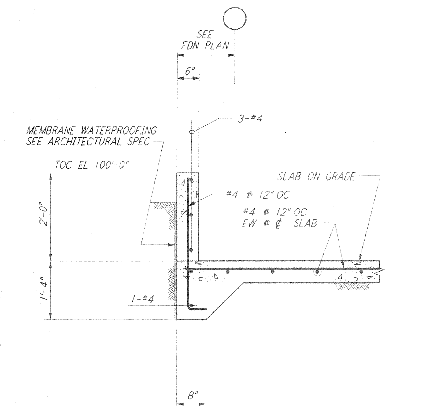
SECTION F REF \frac{3}{4}'' = 1'-0'' WA-S-405 WA-S-102
