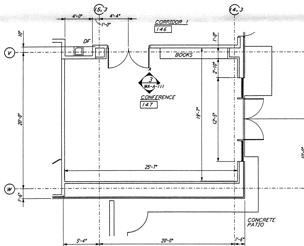
ENLARGED PLAN
