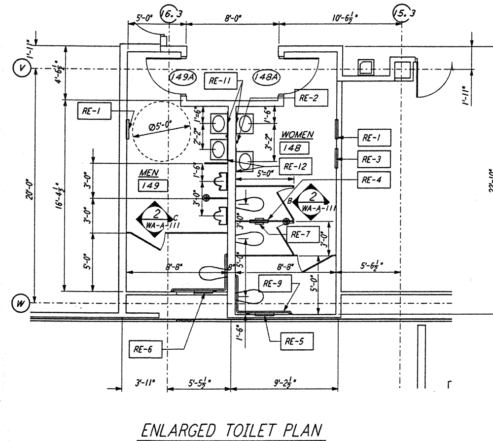
MEN 149 / WOMEN 148 1/4" = 1'-0"
