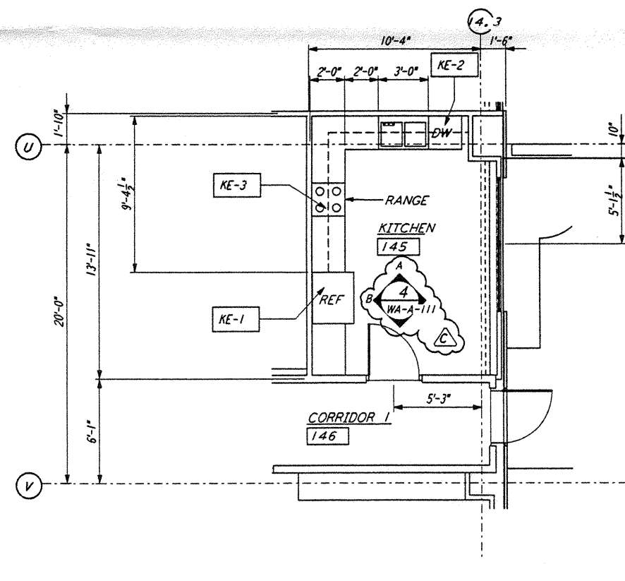
ENLARGED KITCHEN PLAN
