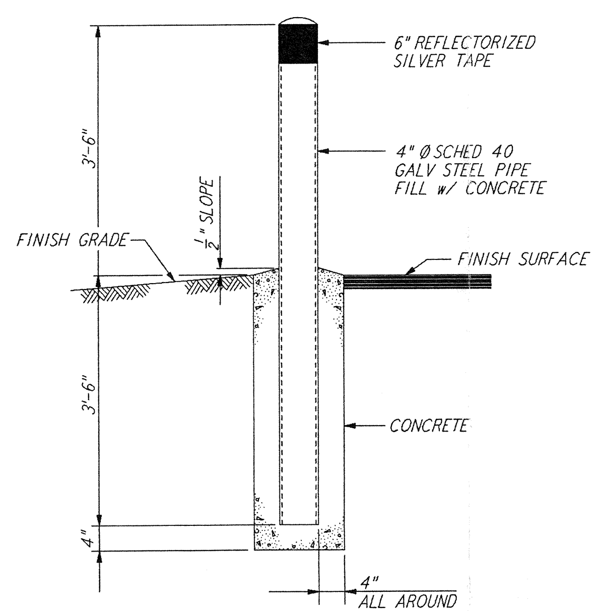
GUARD POST NOT TO SCALE REF: WA-C-055
