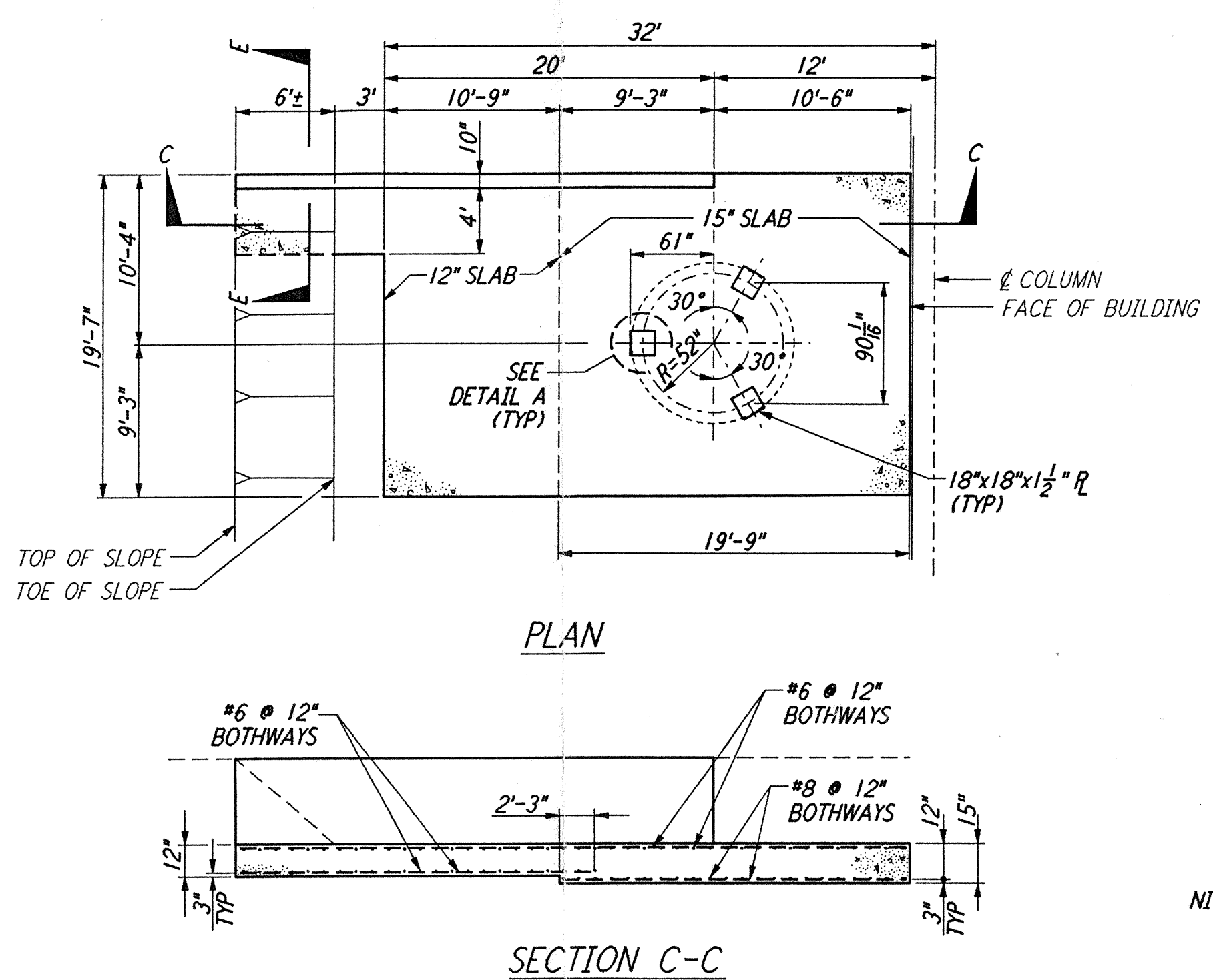
CONCRETE FOUNDATION FOR LIQUID NITROGEN TANK NOT TO SCALE NORTHWEST ARM ONLY SOUTHWEST ARM BY OTHERS REF: WA-C-021, WA-C-025, WA-C-041, WA-C-045, WA-C-505
