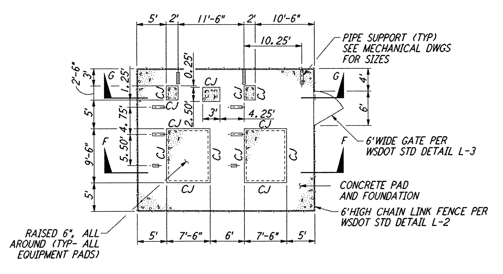
ENLARGED CHILLER YARD PLAN @ MID AND END STATIONS NOT TO SCALE REF: WA-C-021, WA-C-025, WA-C-041, WA-C-045 NOTE: FOR MID AND END STATIONS - NORTHWEST ARM, USE PLAN AS SHOWN. FOR MID AND END STATIONS - SOUTHWEST ARM, PLAN IS ROTATED 90° AND MIRRORED ABOUT THE BEAM TUBE.
