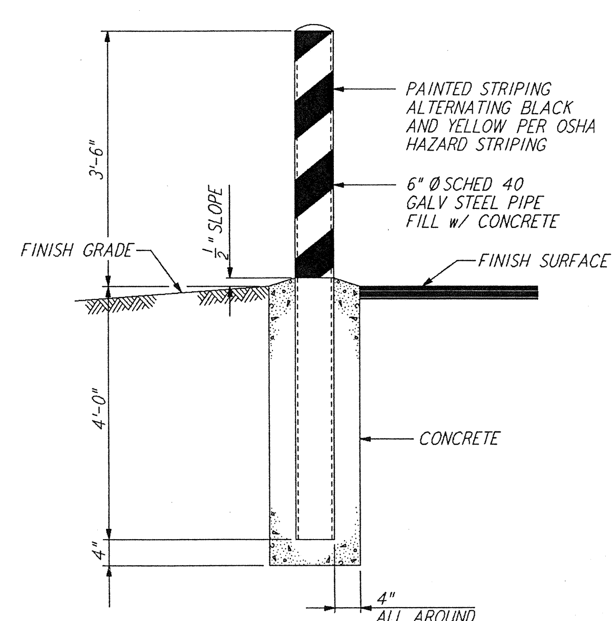
BOLLARD NOT TO SCALE REF: WA-C-006, WA-C-021, WA-C-025, WA-C-041, WA-C-045, WA-C-505
