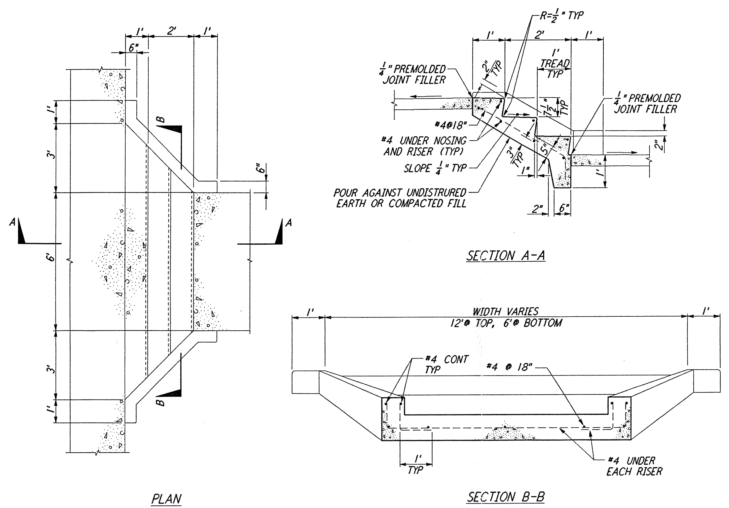
CONCRETE STEPS NOT TO SCALE REF: WA-C-006, WA-C-005
