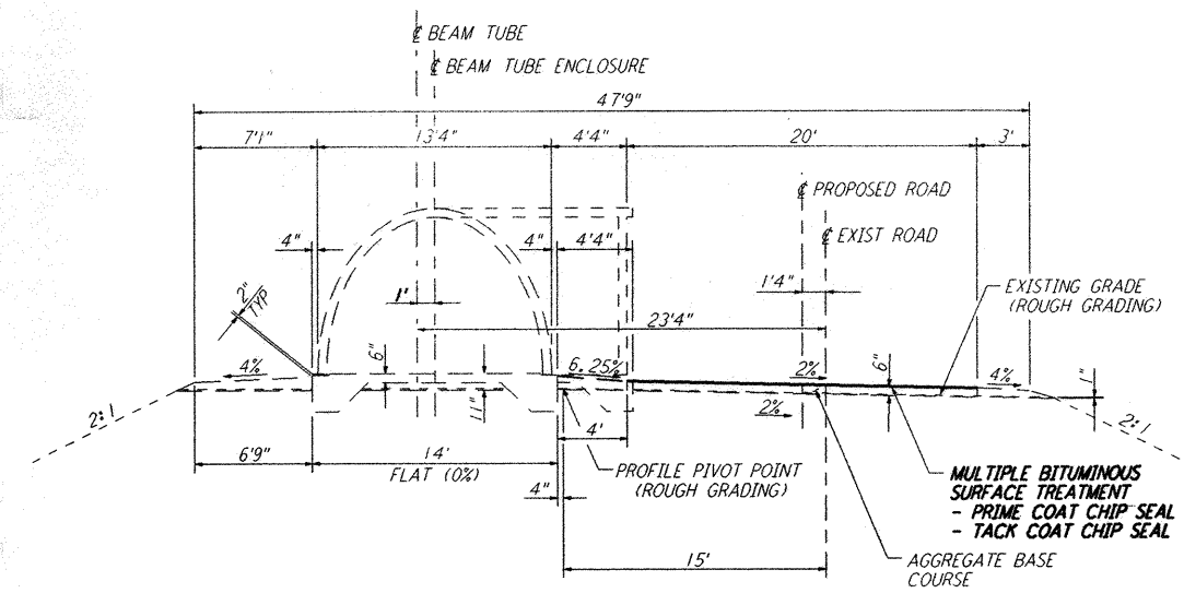
SECTION A NOT TO SCALE WA-C-004
