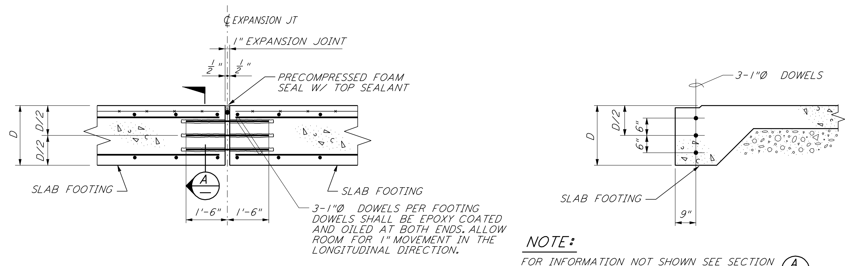
TYPICAL EXPANSION JOINT AT SLAB FOOTING
