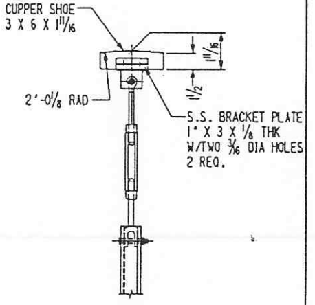
SIDE VIEW REPAIR JACK
