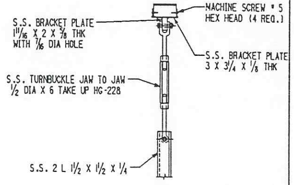
ELEVATION VIEW REPAIR JACK
