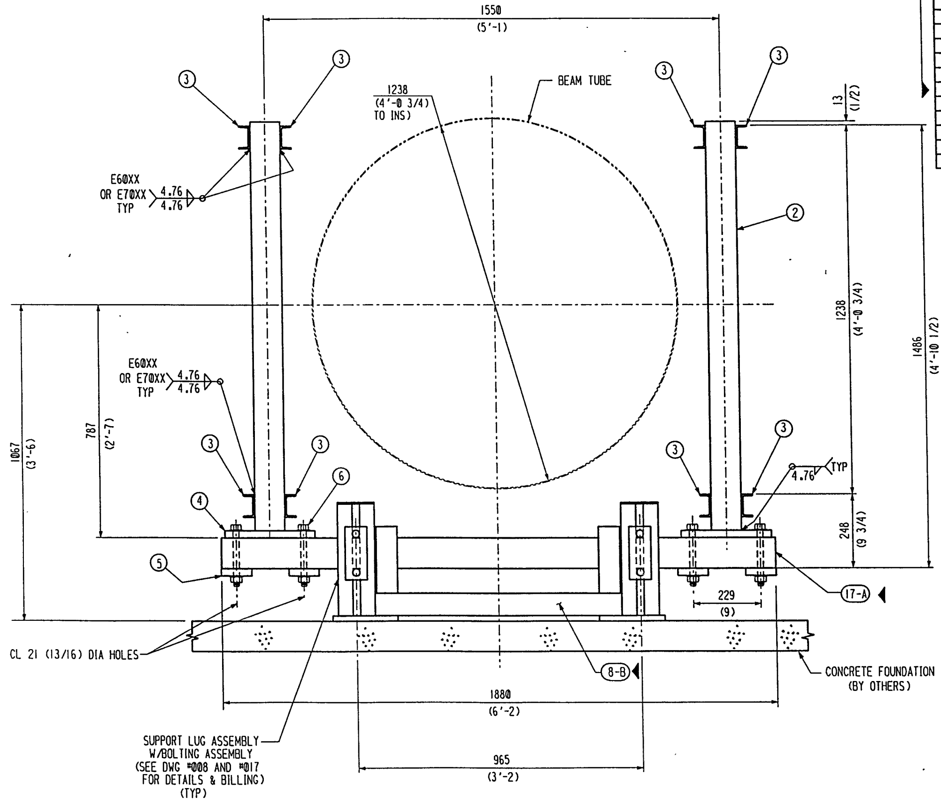
SECTION 8-B (FROM DWG #017) (SECTIONS NOT SHOWN FOR CLARITY)
