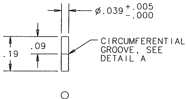
-1. WIRE RELEASE ROD SCALE: 4/1
