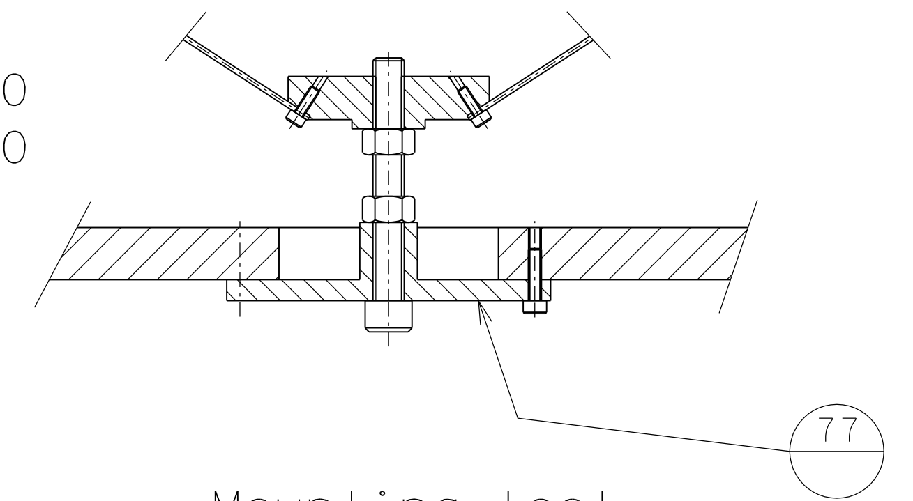
Mounting tool
