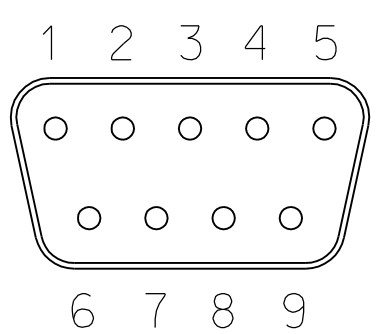
Accu-Glass 9D-10400 9 pin sub-D male connector on stand
