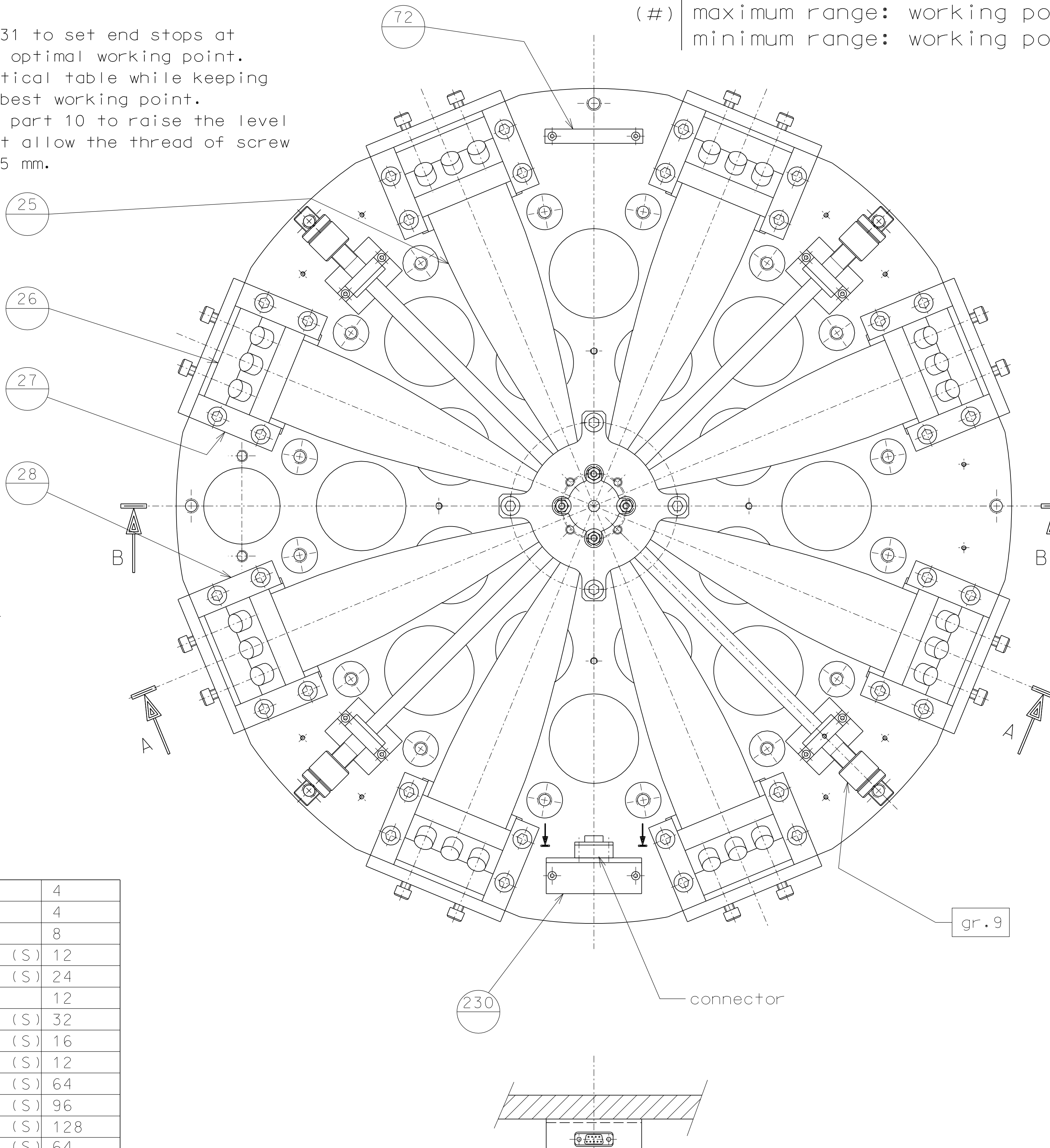
bunting magnetics N30P750250500-SH 8 magnets per filter maximum baking temperature 145 °C
