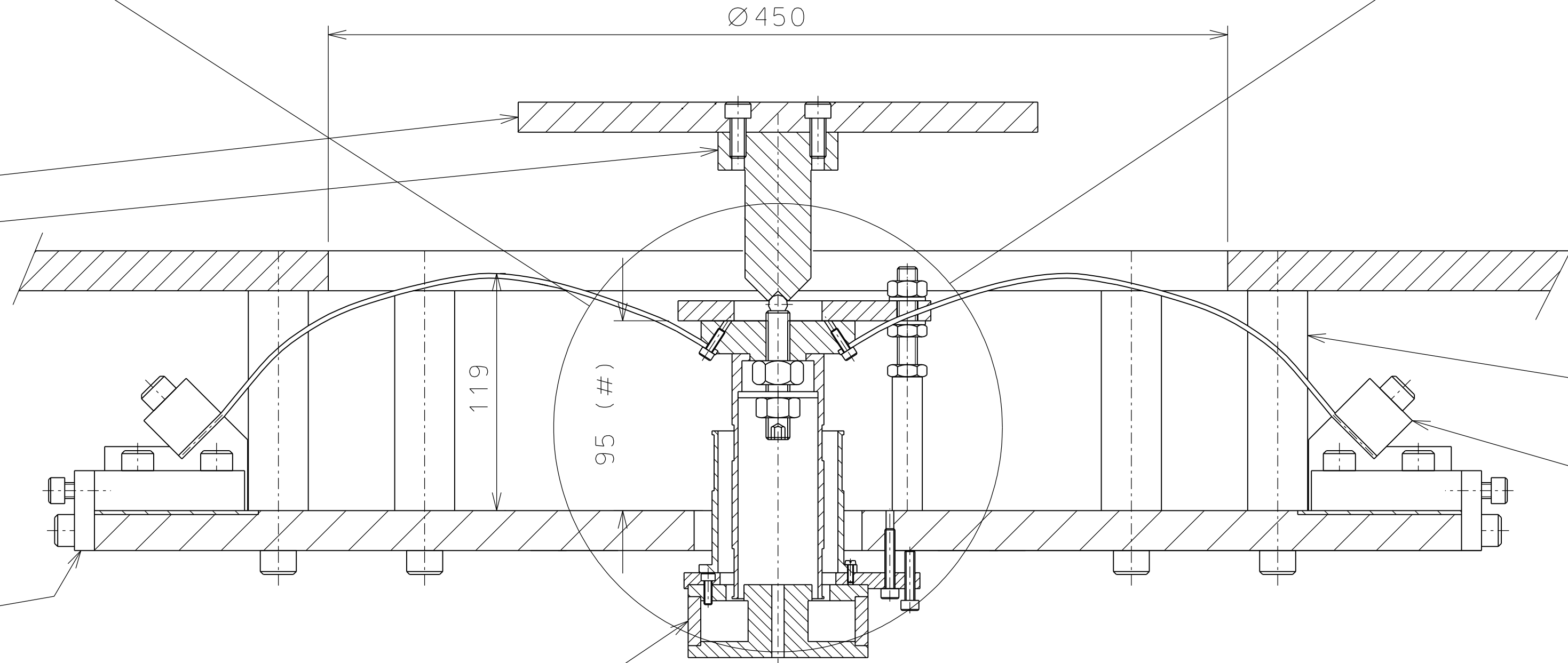
bunting magnetics N30P750250500-SH 8 magnets per filter maximum baking temperature 145 °C
