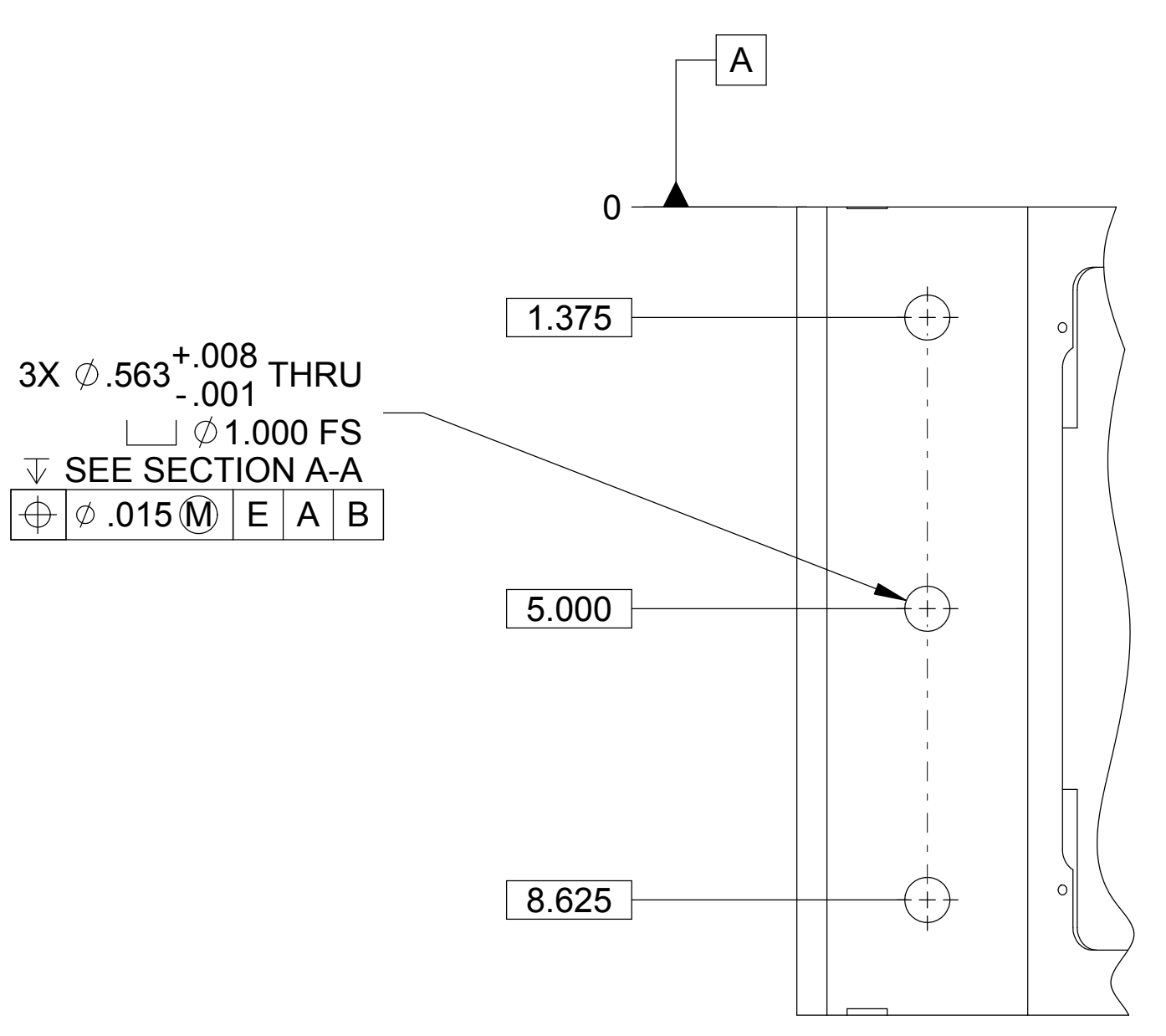
VIEW F-F
