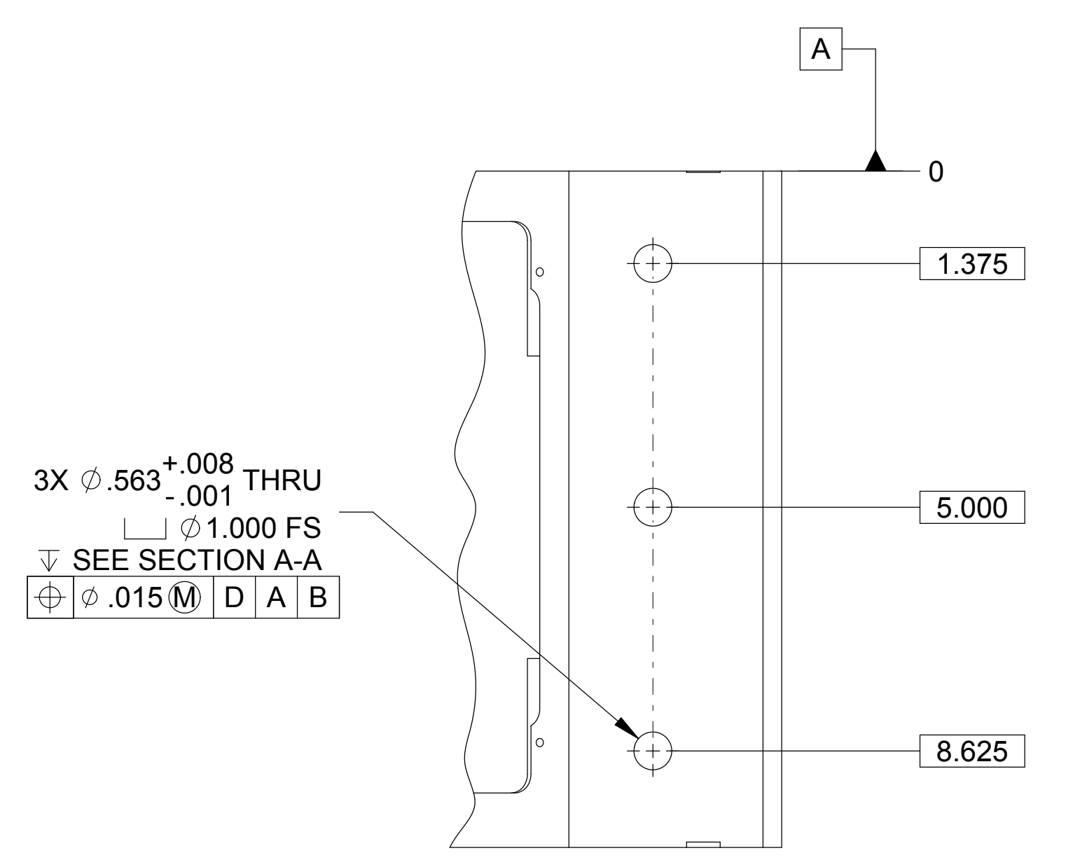
VIEW E-E
