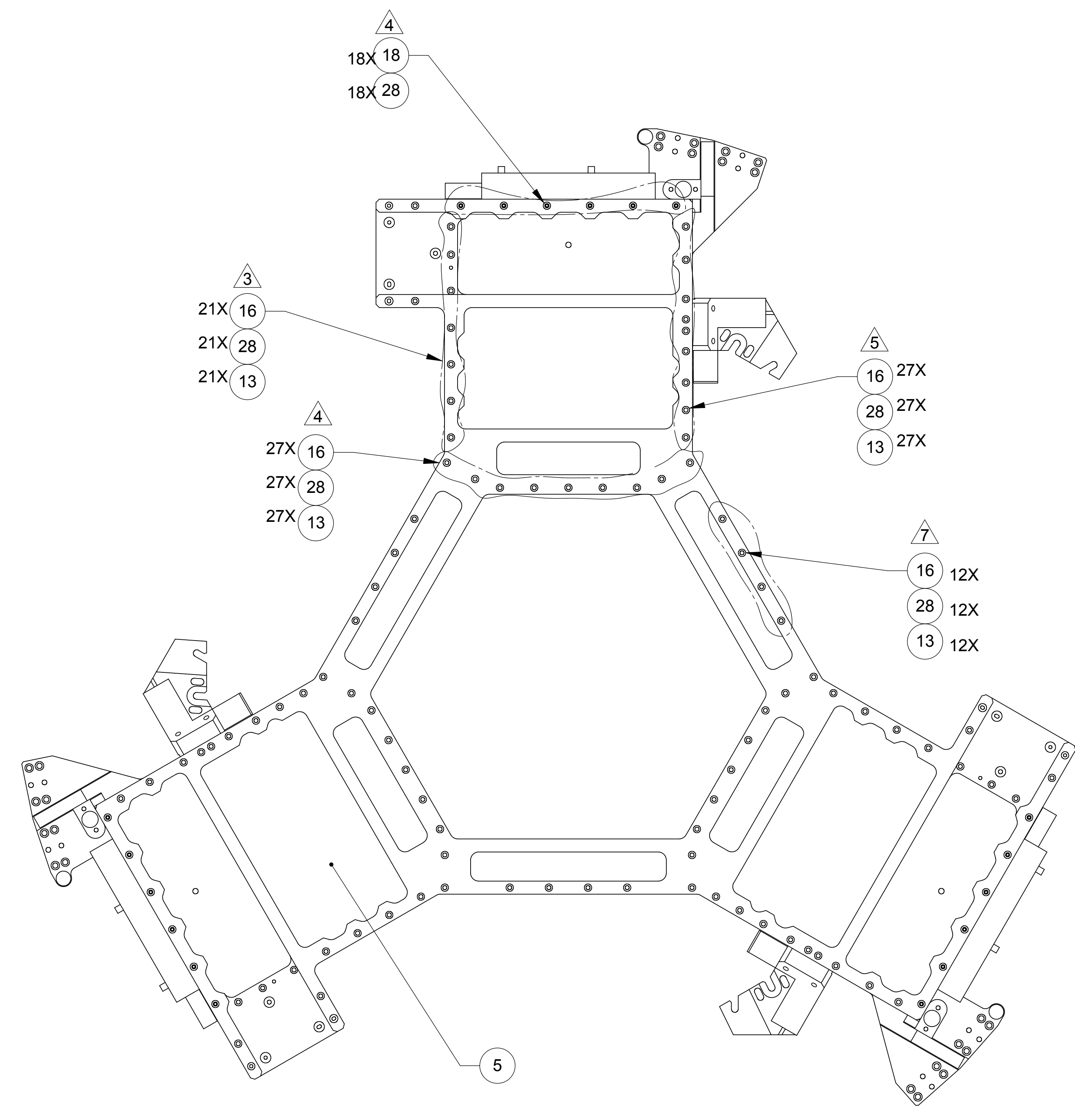
TOP VIEW
