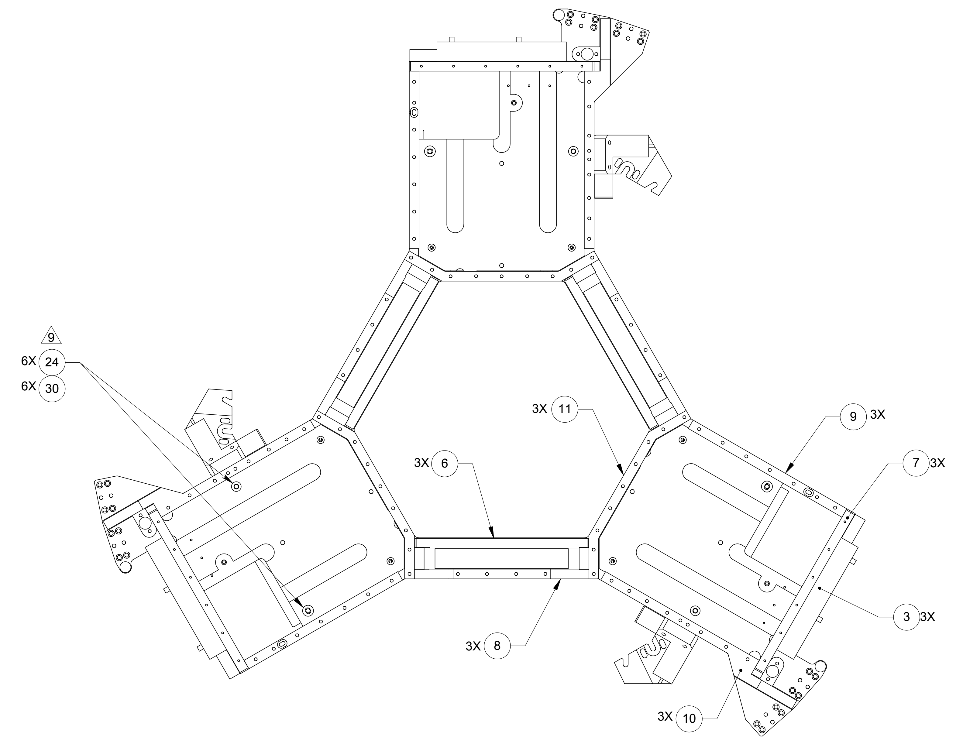
TOP VIEW ITEM 5 CLOSEOUT PLATE REMOVED
