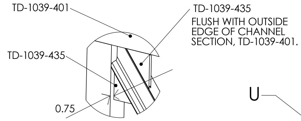
DETAIL U SCALE 1 : 6
