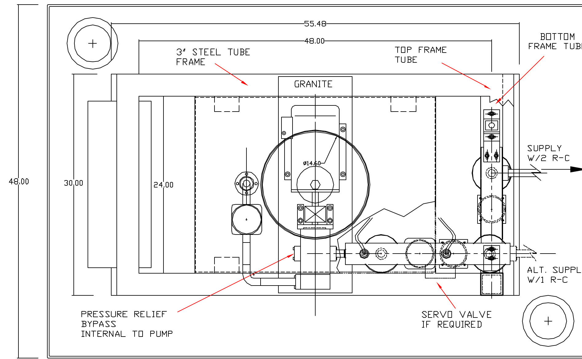
PUMP STATION TOP VIEW
