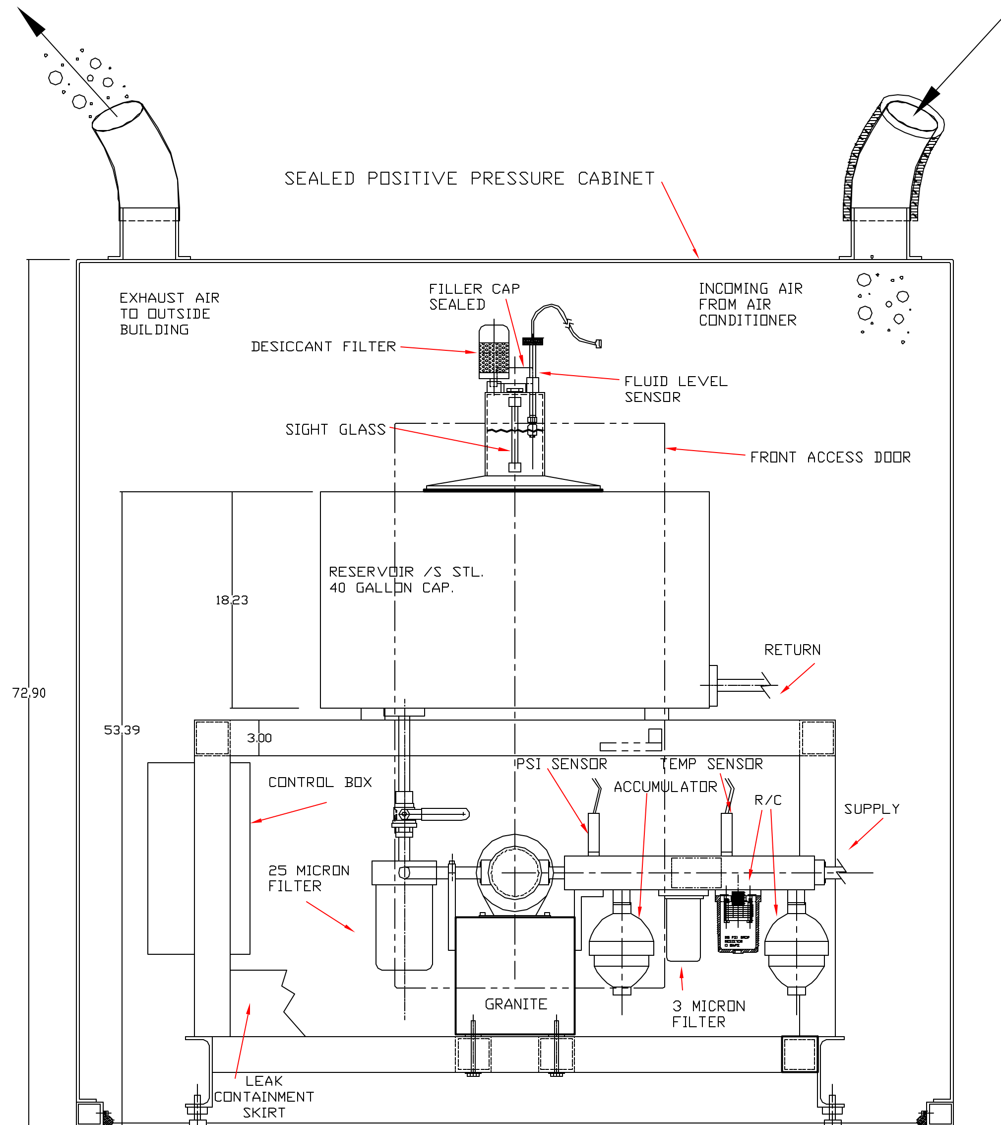
PUMP STATION FRONT VIEW
