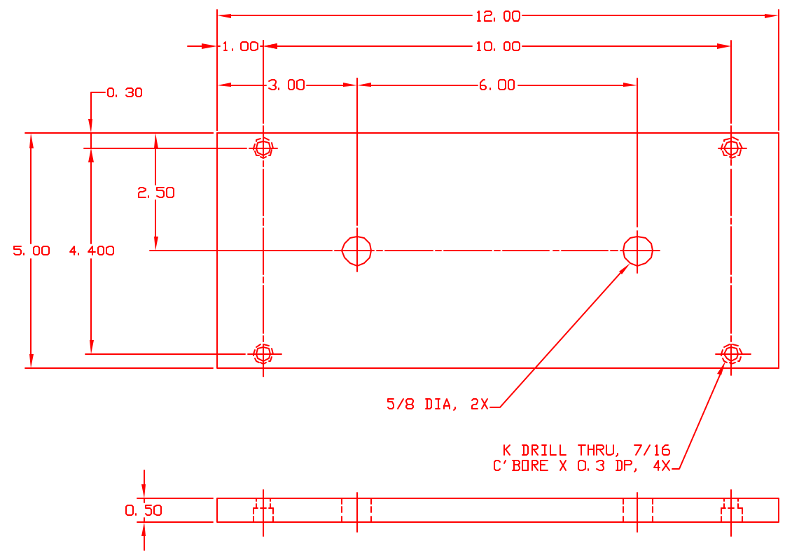
BASE 1 REQ' D. MAT' L: 6061-T6 ALUMINUM
