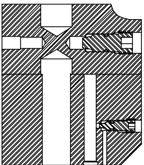
SECTION BW-BW
