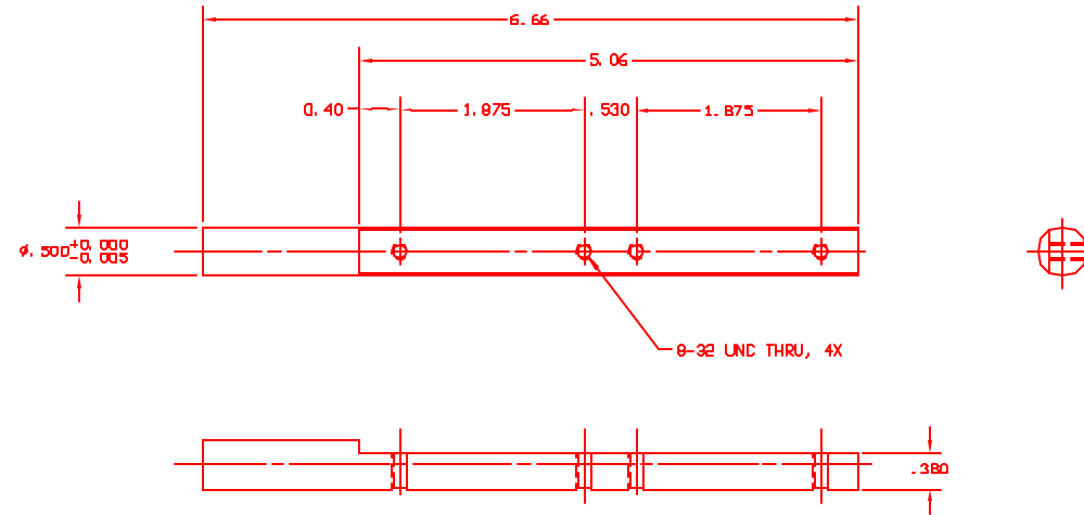
-1. SHAFT, MIRROR HOLDER MATERIAL: SST SHAFTING
