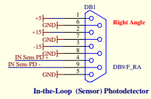
In-the-Loop (Sensor) Photodetector
